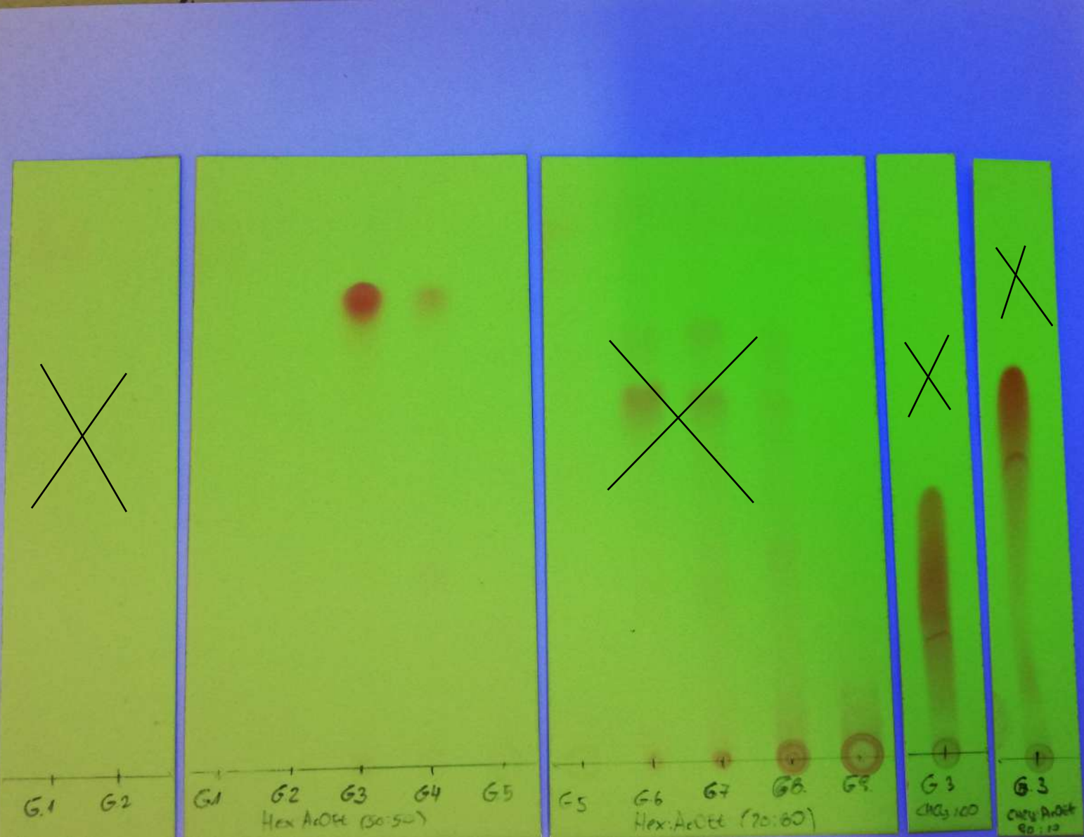
FIG 5 a (TLC plate under UV-light)
