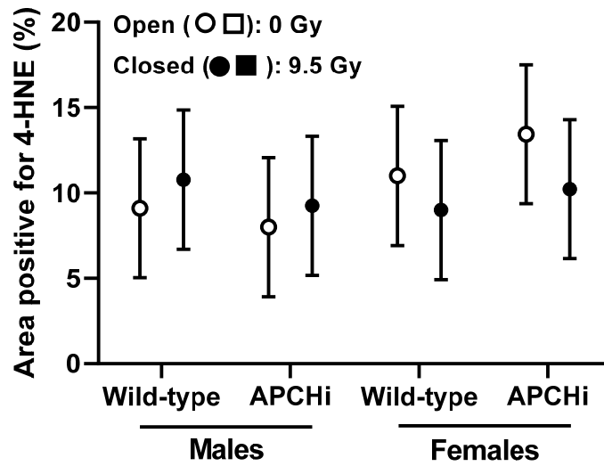
S15 Fig. Epidermal are positive for 4-HNE. Positivity for 4-HNE was assessed with immunohistochemistry. Graphs indicate means and SD of the statistical model; n=6-9 wild-type males in 0 Gy, 10 wild-type males in 9.5 Gy, 6-8 APCHi males in 0 Gy, 8-9 APCHi males in 9.5 Gy, 7-8 wild-type females in 0 Gy, 5-6 wild-type females in 9.5 Gy, 8-9 APCHi females in 0 Gy, and 8-9 APCHi females in 9.5 Gy.
