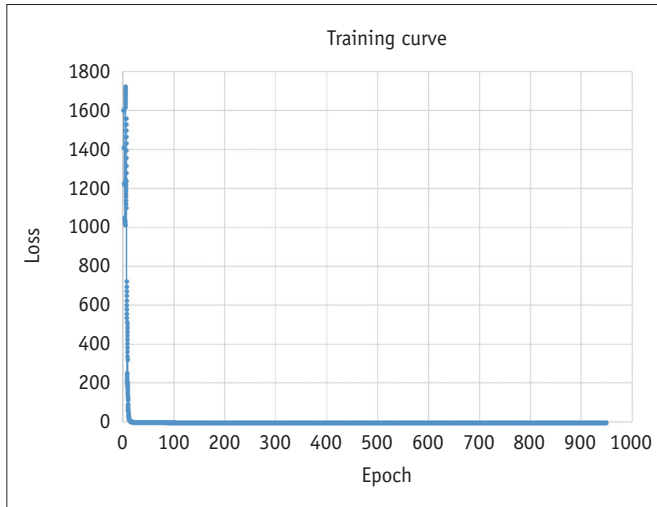
Supplementary Fig. 1. Training loss curve of YOLOv3.
