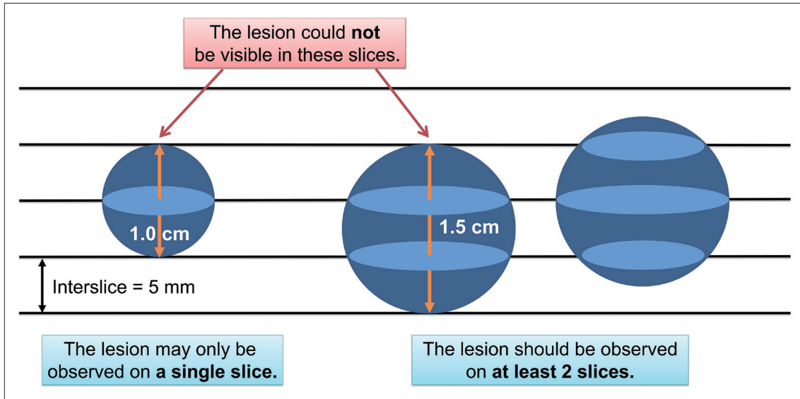
Supplementary Fig. 2. Theoretical background of the false positive filtering method.
