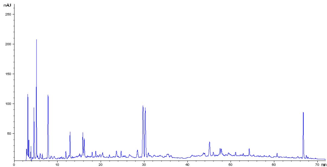
Supplementary figure 1 Chromatogram of Guhong injection (GHI) by injection by HPLC analysis at the UV detection wavelength of 280 nm.
