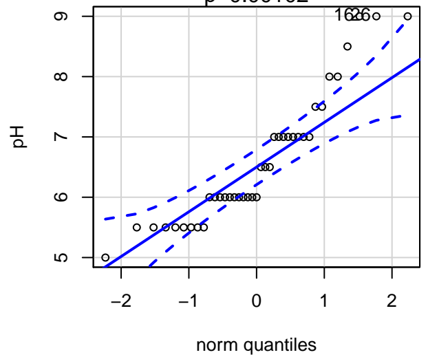
p=0.00102
