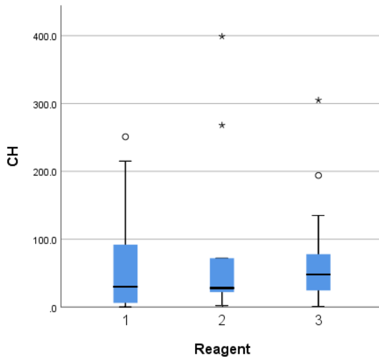
Supplemental Figure S2 - Box and whiskers plot displaying resting serum bile acid concentrations (Y-axis, in \mu\text{mol/L} ) in dogs with chronic hepatitis measured using the three different reagents, Dialab (1), Randox (2) and Sentinel (3). The horizontal black line in the boxes represents the median serum bile acid concentrations. CH, chronic hepatitis.
