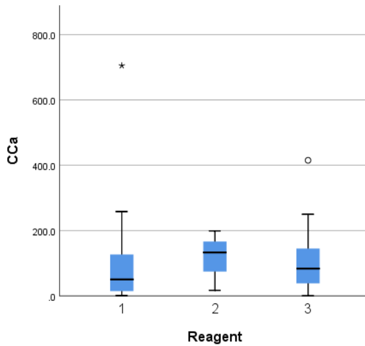
Supplemental Figure S4 - Box and whiskers plot displaying resting serum bile acid concentrations (Y-axis, in \mu\text{mol/L} ) in dogs with congenital circulatory anomalies measured using the three different reagents, Dialab (1), Randox (2) and Sentinel (3). The horizontal black line in the boxes represents the median serum bile acid concentrations. CCa, congenital circulatory anomaly.
