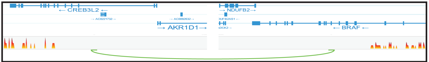
Supplemental Figure 3: Linked read genome sequencing identifies structural variations in the MDA8788-6 genome involving ZNF546 and AXL as well as CREB3L2 and BRAF.
