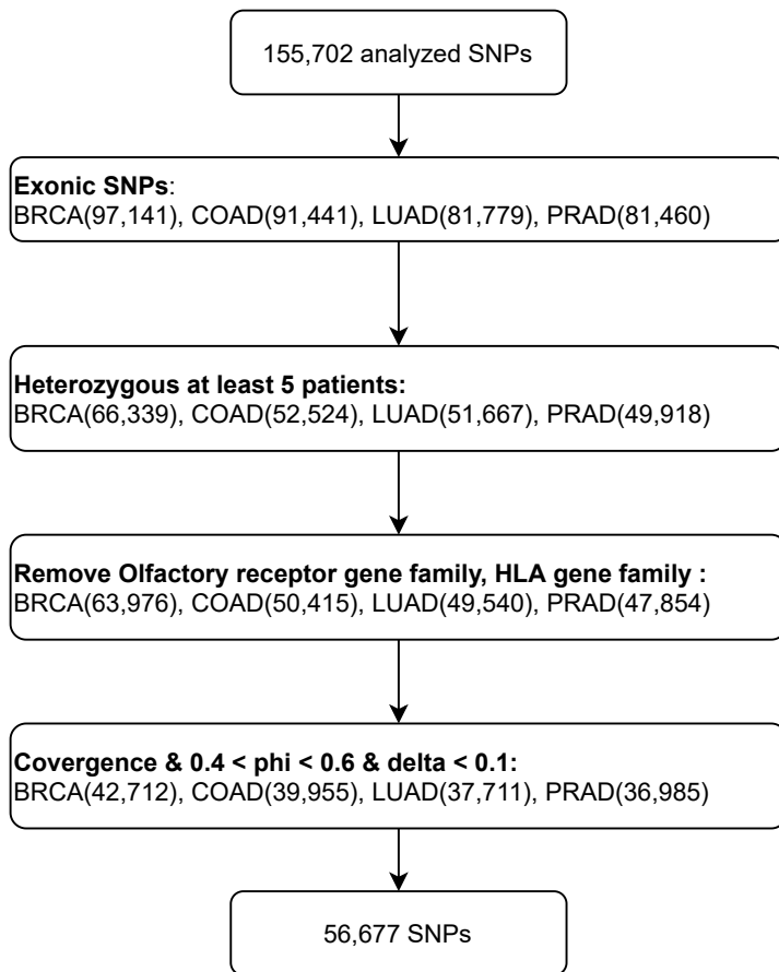
Fig. S1. The inclusion and exclusion filtering of exonic SNPs for allelic imbalance analysis in four cancer types.
