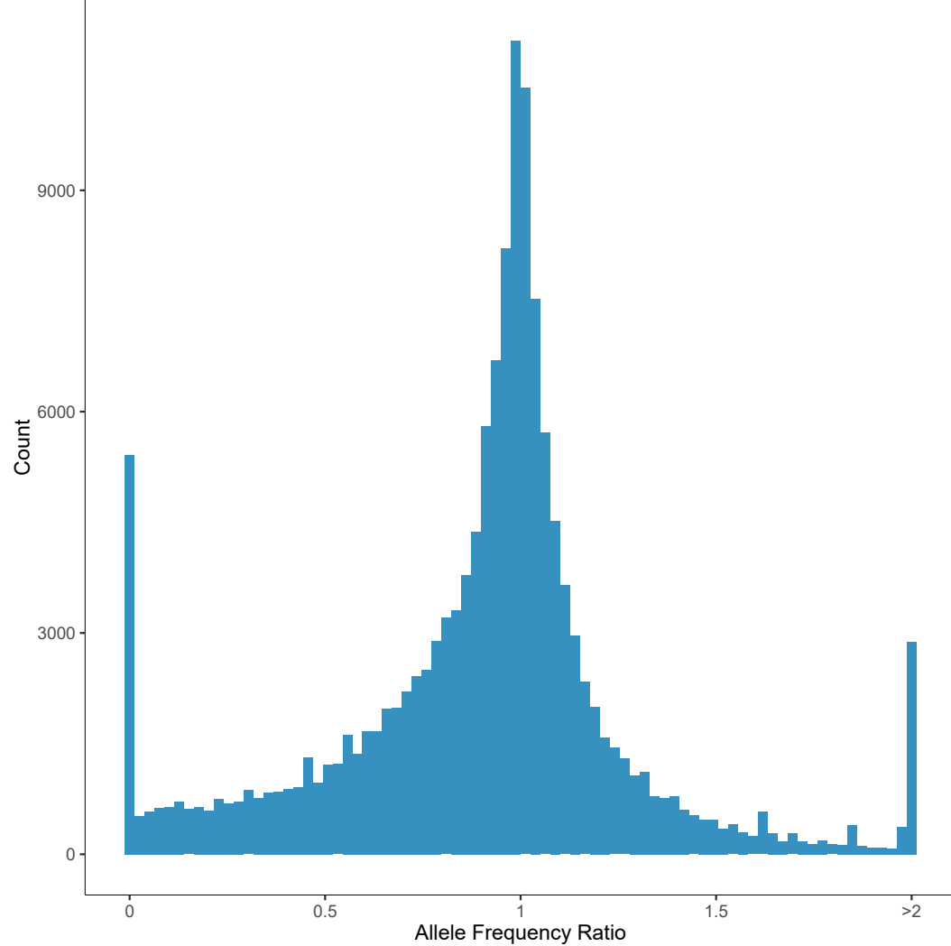
Fig. S2. The distribution of allele frequencies (a) and the ratios of allele frequencies (b) of exonic SNPs in four cancer types.
