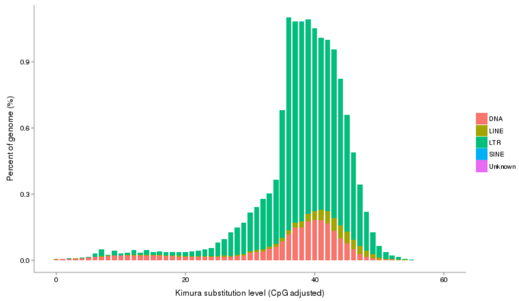
Supplemental Figure 3: The distribution of TE (tandem repeat elements) sequence divergence of the C. chinensis genome.
