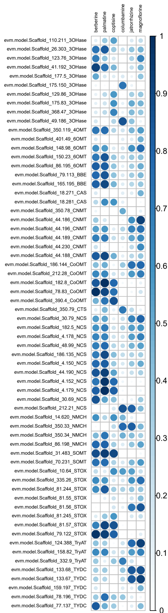
Supplemental Figure 7. Coefficient of determination ( R^2 ) between candidate genes and contents of various alkaloids in C. chinensis .
