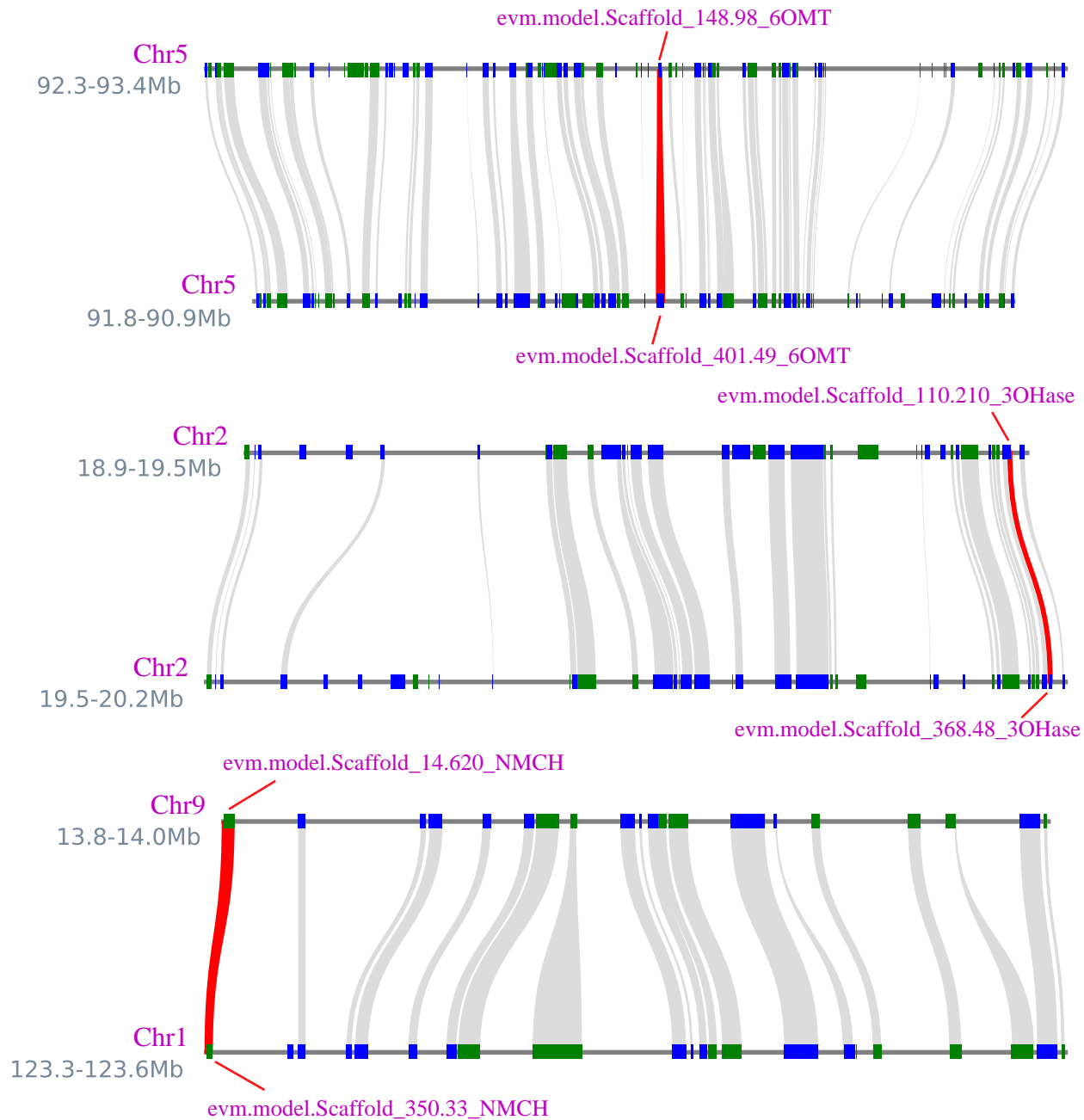
Supplemental Figure 8. Recently duplicated genes blocks, where genes involved in BIAs synthesis are located.
