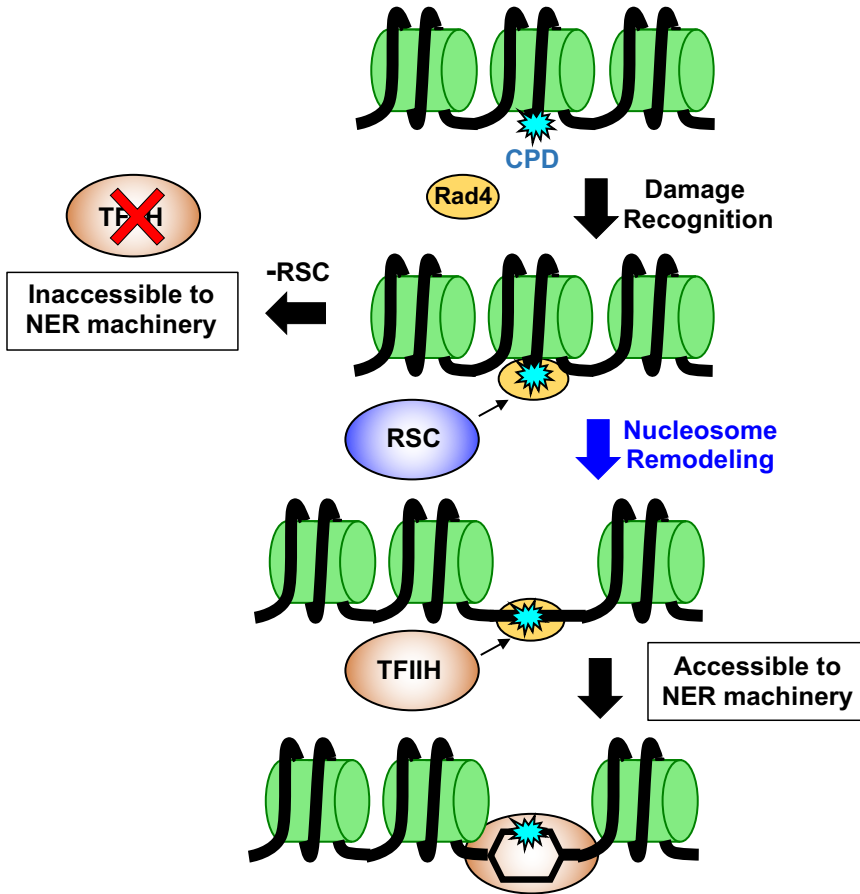
Supplemental Figure S13: Model of how RSC may facilitate repair of CPD lesions in nucleosomes by shifting or evicting the associated nucleosome to promote TFIIH recruitment. See also Fig. 7.
