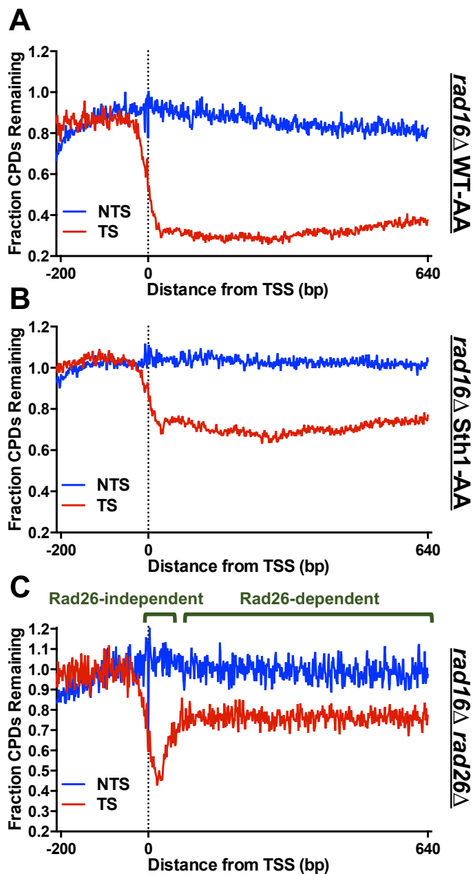
Supplemental Figure S6: Sth1-AA depletion effects both Rad26-dependent and Rad26-independent TC-NER. ( A-C ) CPD-seq analysis examining the repair of CPDs on both DNA strands across ~5200 yeast genes relative to the transcription start site (TSS) following 2hr repair in ( A ) rad16 Δ WT-AA, ( B ) rad16 Δ Sth1-AA, and ( C ) rad16 Δ rad26 Δ. CPD-seq data for rad16 Δ rad26 Δ was originally published in (Duan et al. 2020).
