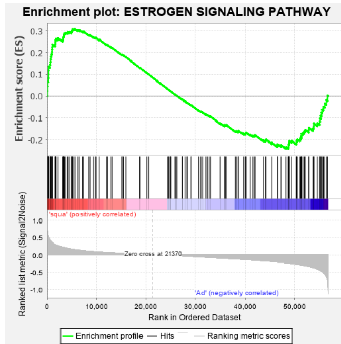
Supplementary Figure 5. Gene set enrichment analysis (GSEA) of cervical squamous cell carcinomas (SCC) samples from our study. Genes enriched in cervical SCC that participate in estrogen signaling pathway were identified by GSEA software [12].
