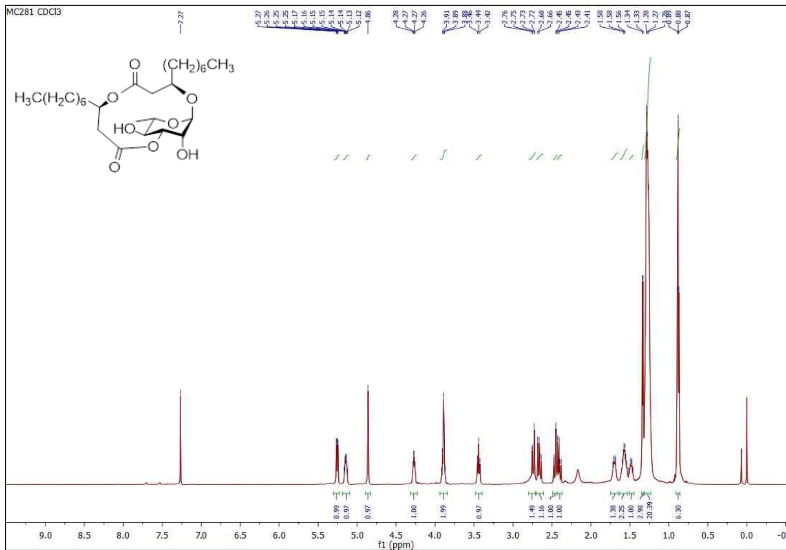
Figure S206 | ^1\text{H} NMR spectrum ( \text{CDCl}_3 , 600 MHz) of (1 \rightarrow 3)-macrolactonized rhamnolipid 6a .
