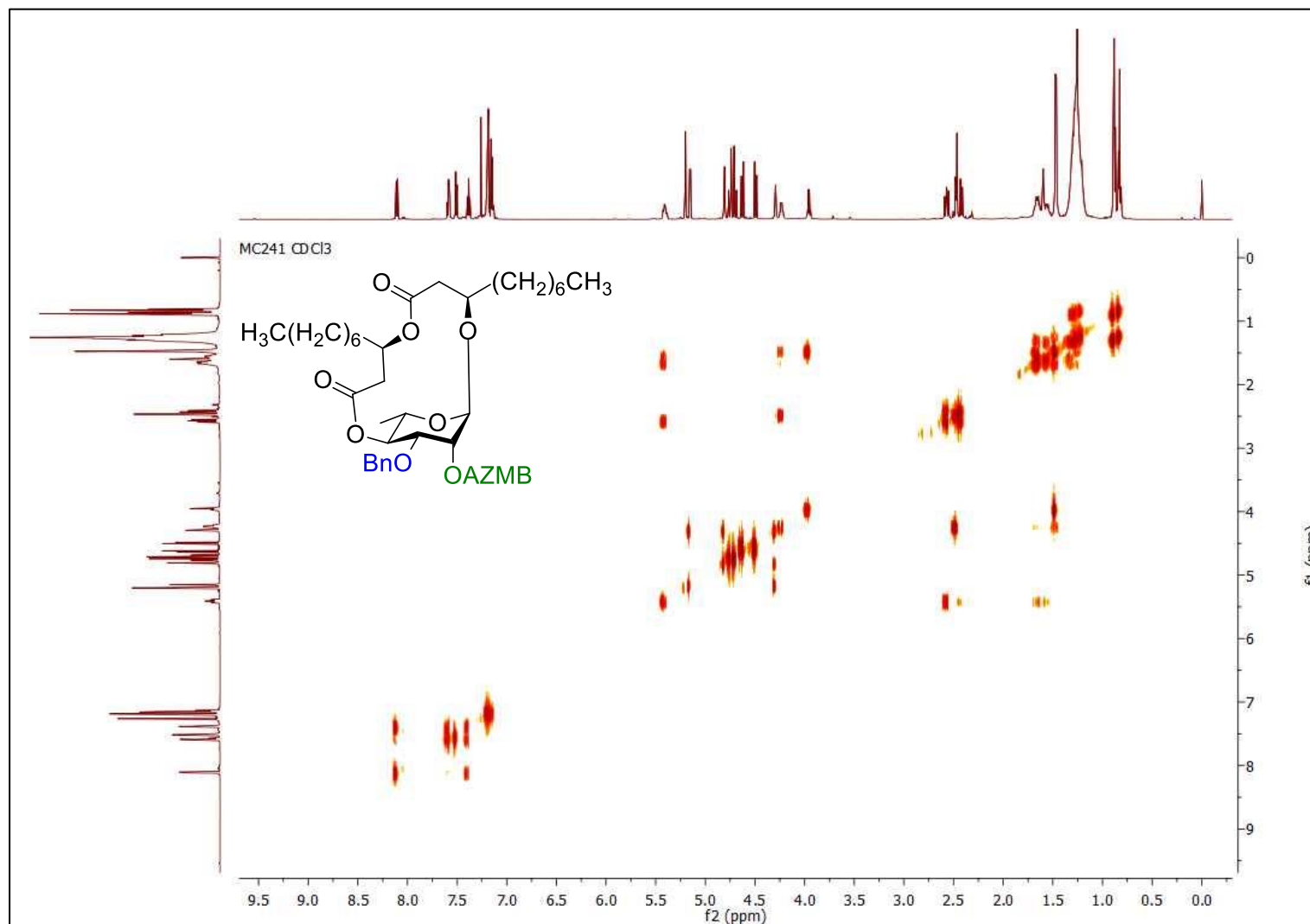
Figure S134 | COSY NMR spectrum (CDCl 3 , 600 MHz) of macrolide 35 .
