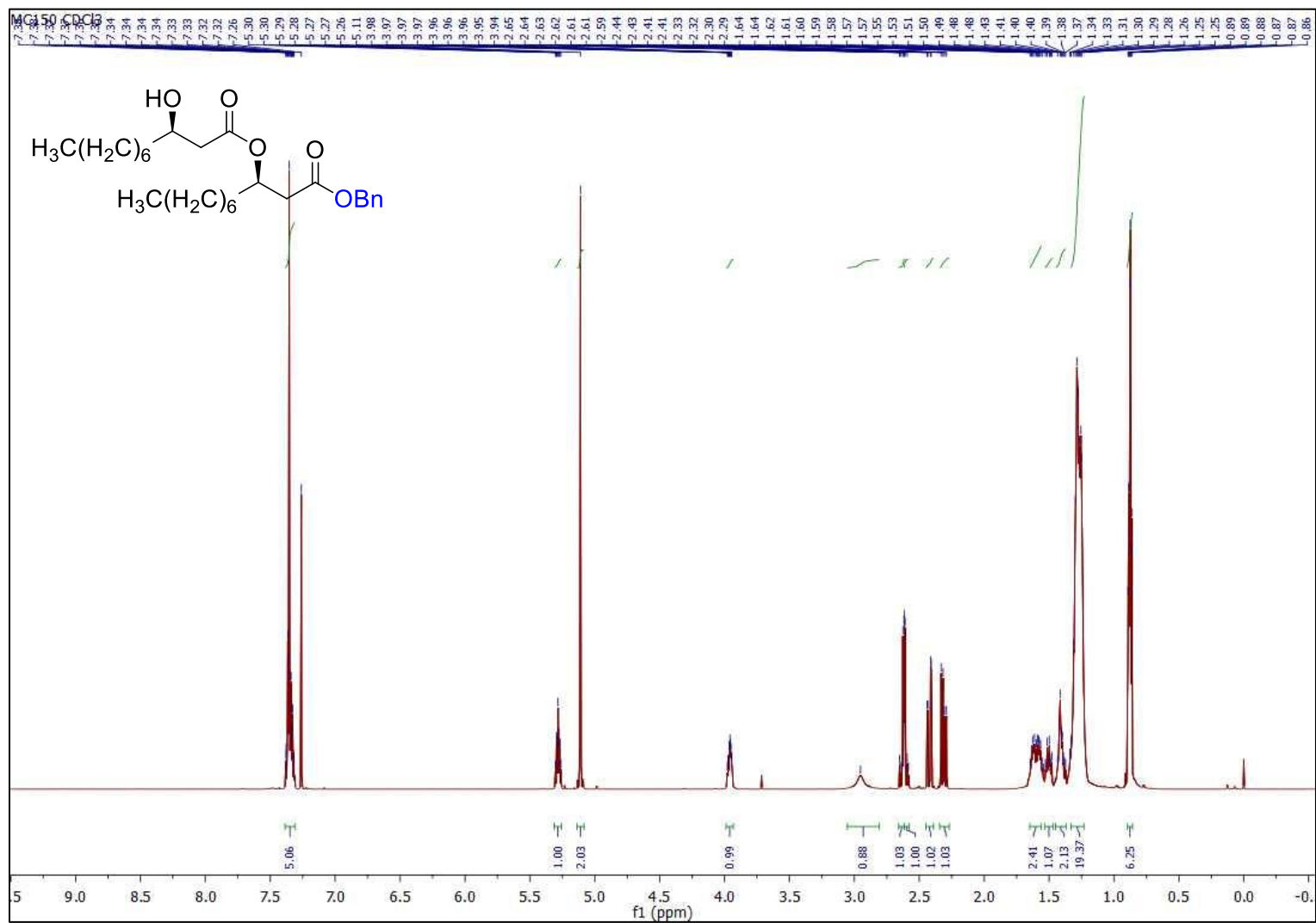
Figure S21 | ^1\text{H} NMR spectrum ( \text{CDCl}_3 , 600 MHz) of ( R )-benzyl 3-((( R )-3-hydroxydecanoyl)oxy)decanoate ( 12 ).
