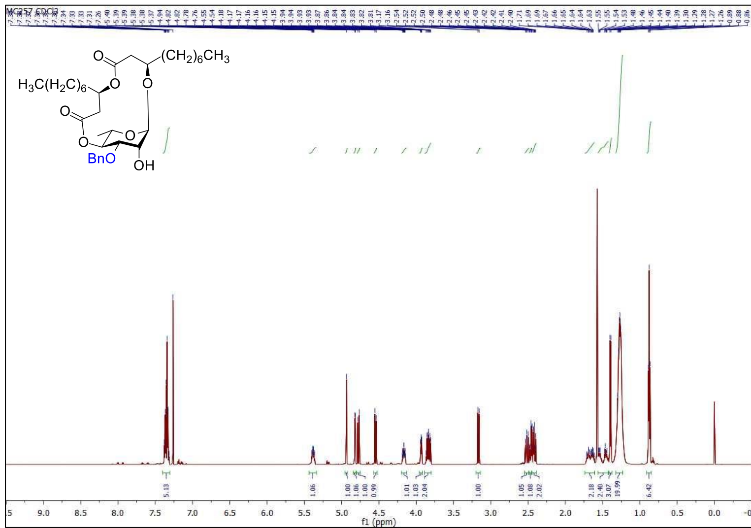
Figure S138 | ^1\text{H} NMR spectrum ( \text{CDCl}_3 , 600 MHz) of macrolide S16.
