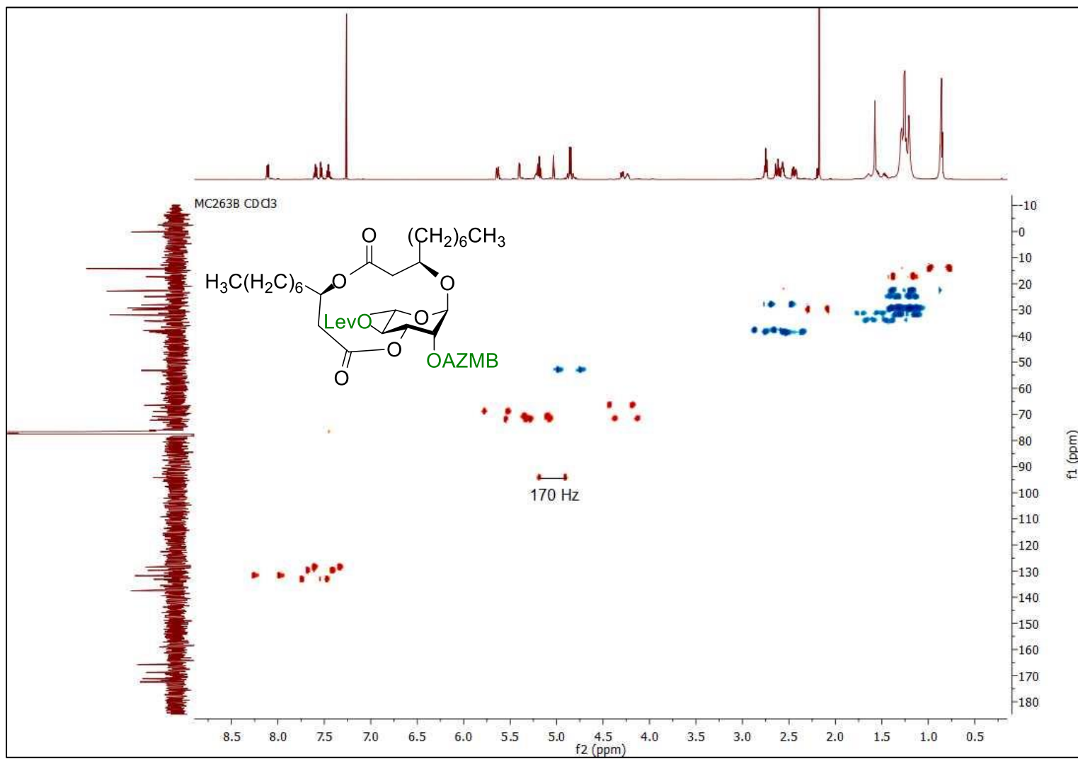
Figure S193 | undecoupled HSQC NMR spectrum (CDCl 3 , 600 MHz) of macrolide 39a .
