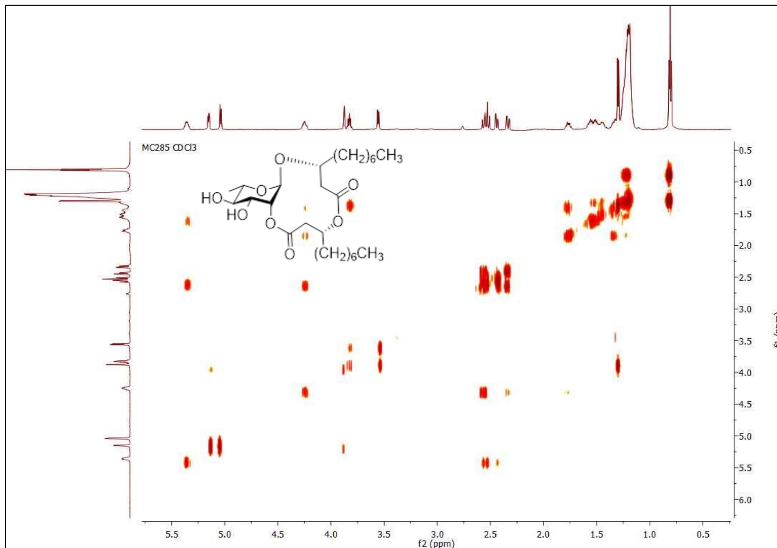
Figure S169 | COSY NMR spectrum (CDCl 3 , 600 MHz) of (1→2)-macrolactonized rhamnolipid 5a .
