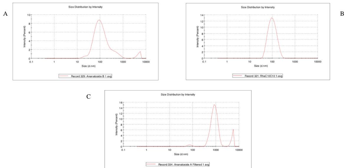
Figure S6. Size distribution of (A) ananatoside B ( 2 ), (B) RhaC 10 C 10 ( 3 ), and (C) ananatoside A ( 1 ) measured by DLS.
