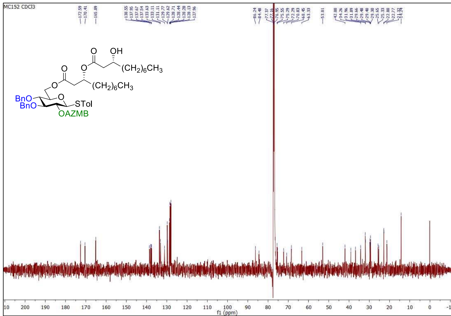
Figure S65 | ^{13}\text{C} NMR spectrum ( \text{CDCl}_3 , 600 MHz) of para -methylphenyl 2- O - ortho -(azidomethyl)benzoyl-3,4-di- O -benzyl-6- O -( R )-3-(( R )-3-(hydroxydecanoyl)oxy)decanoyl-1-thio- \beta -D-glucopyranoside ( 20 ).
