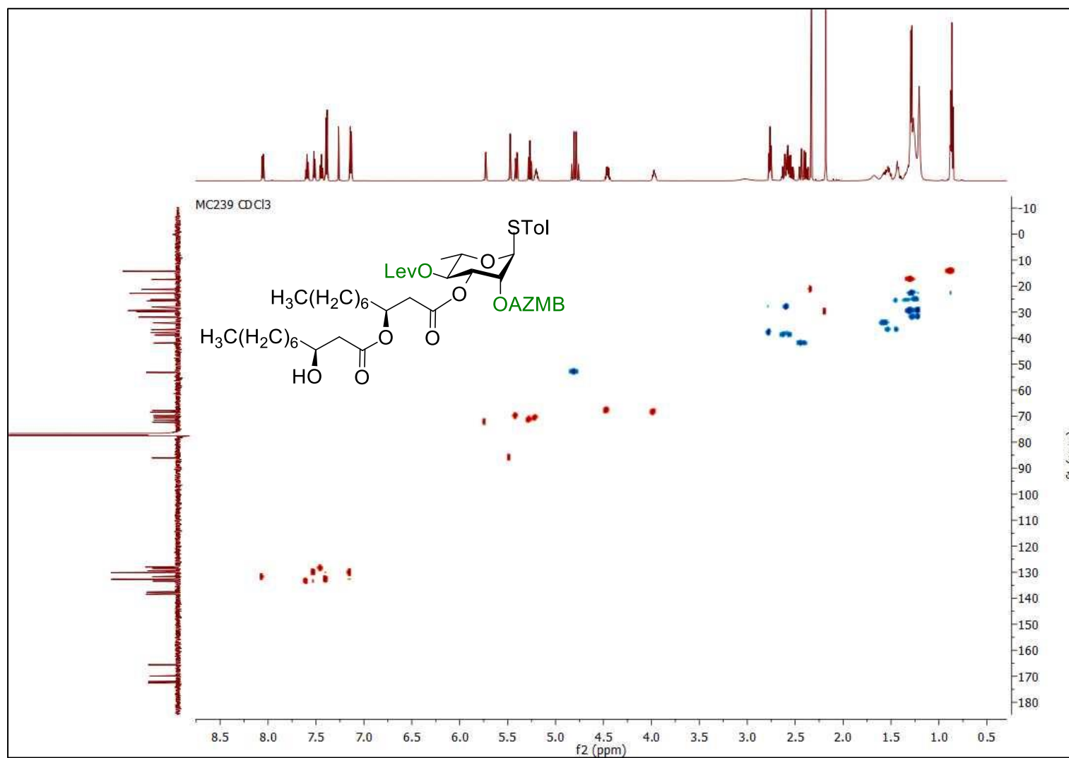
Figure S183 | HSQC NMR spectrum (CDCl 3 , 600 MHz) of para -methylphenyl 2- O - ortho -(azidomethyl)benzoyl-3- O -( R )-3-((( R )-3-(hydroxydecanoyl)oxy)decanoyl-4- O -levulinoyl-1-thio- \alpha -L-rhamnopyranoside ( 38 ).
