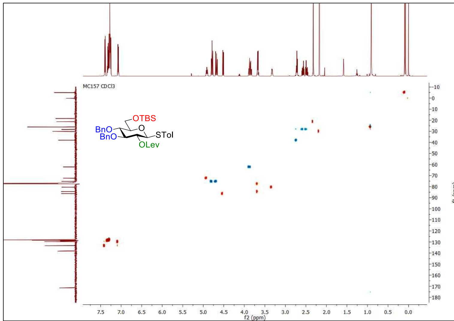
Figure S32 | HSQC NMR spectrum (CDCl 3 , 600 MHz) of para -methylphenyl 3,4-di- O -benzyl-6- O - tert -butyldimethylsilyl-2- O -levulinoyl-1-thio- \beta -D-glucopyranoside ( 11 ).
