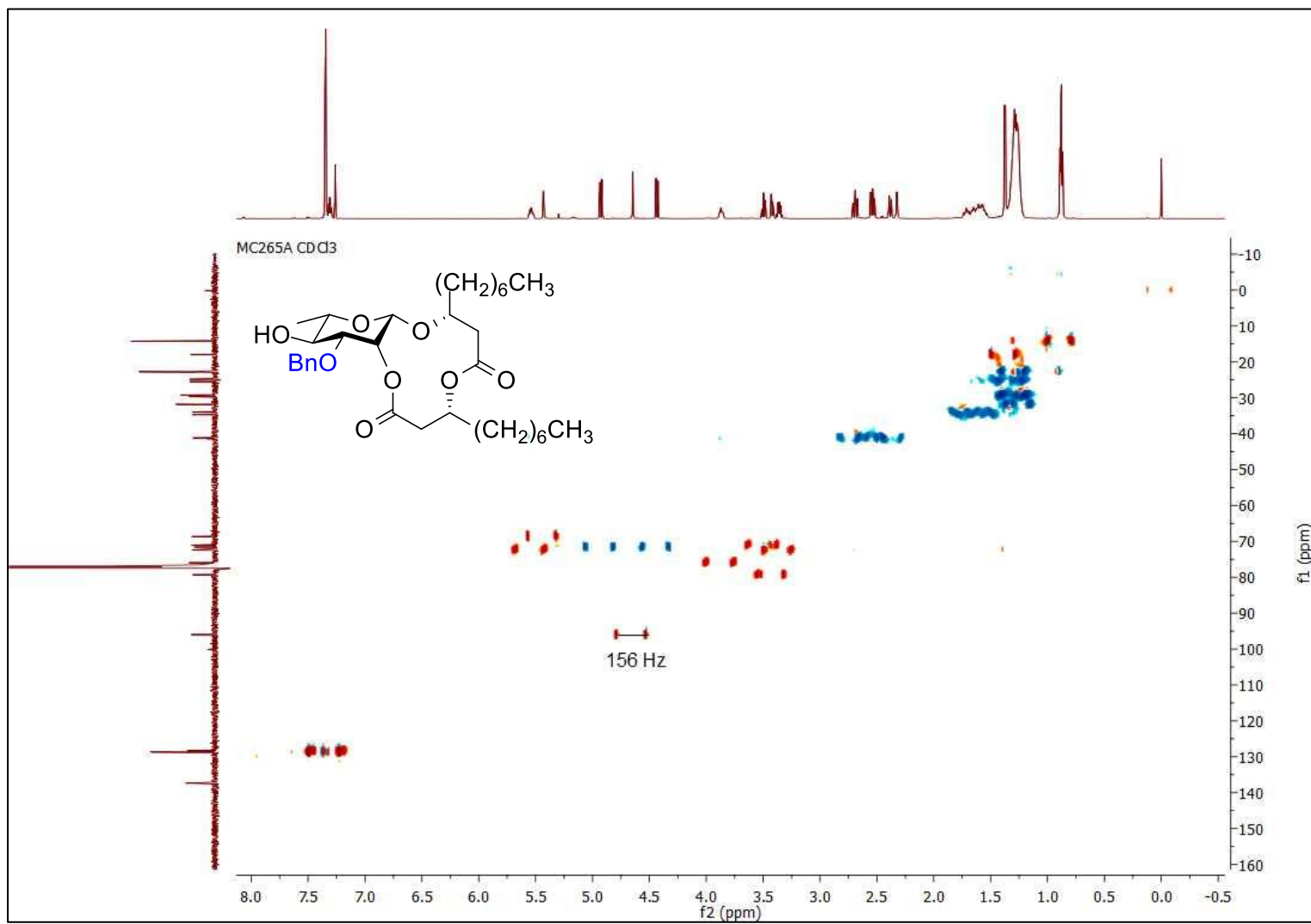
Figure S163 | undecoupled HSQC NMR spectrum (CDCl 3 , 600 MHz) of macrolide S17β .
