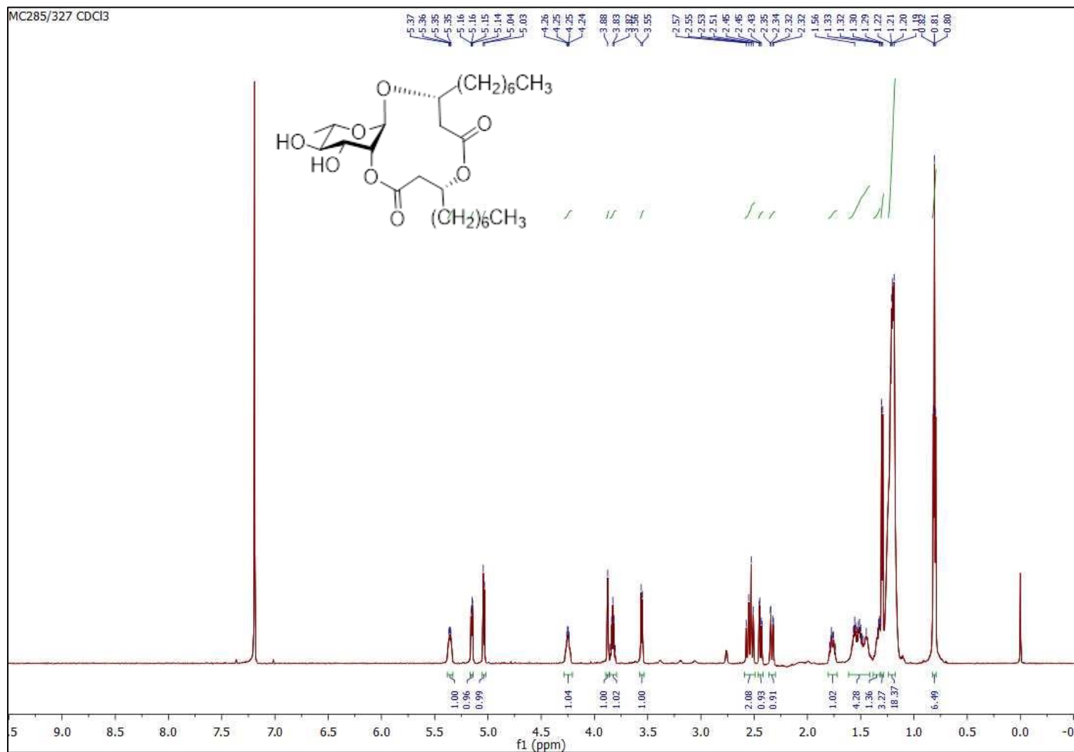
Figure S168 | ^1\text{H} NMR spectrum ( \text{CDCl}_3 , 600 MHz) of (1 \rightarrow 2)-macrolactonized rhamnolipid 5a .
