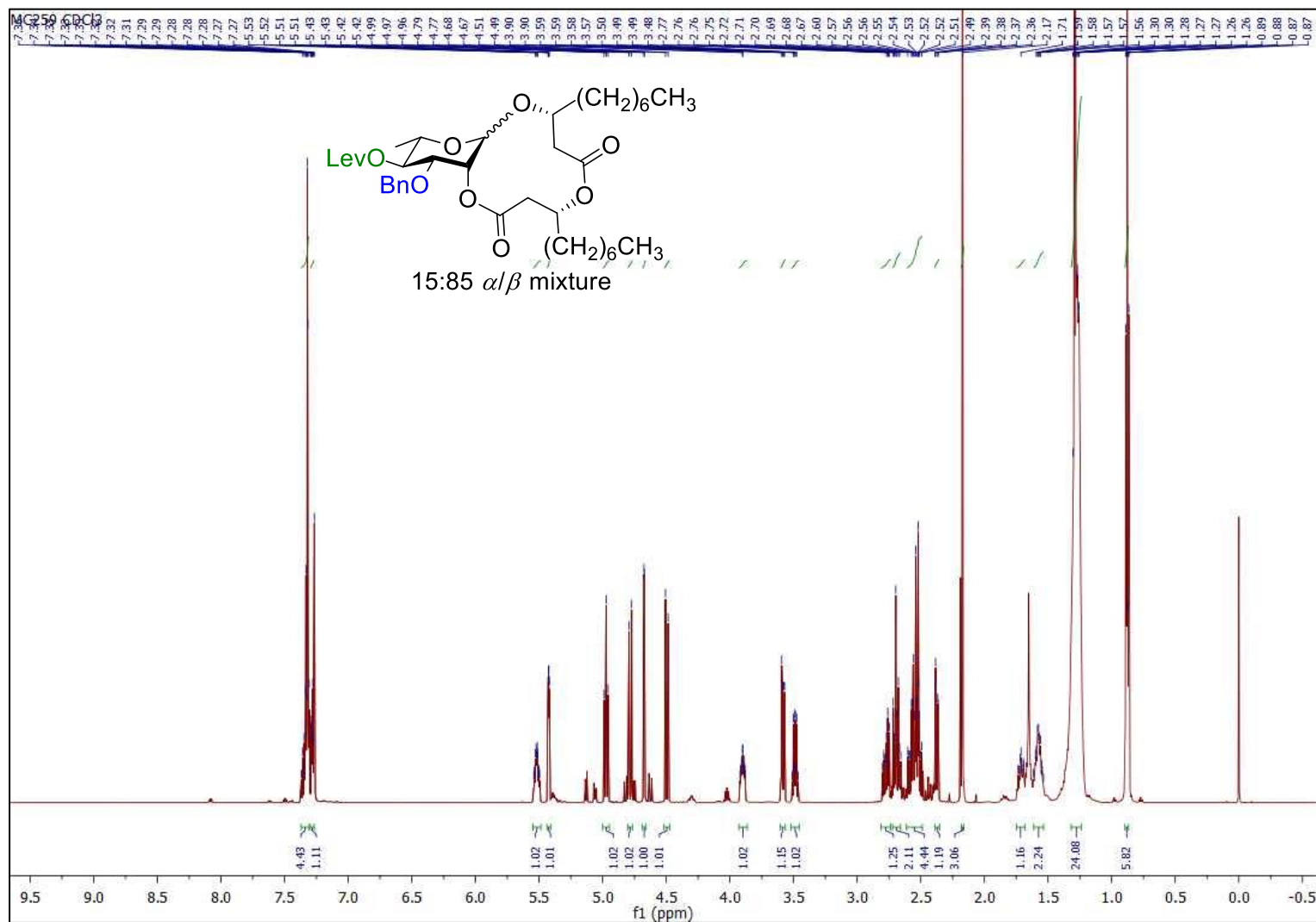
Figure S154 | 1 H NMR spectrum (CDCl 3 , 600 MHz) of macrolide 37 .
