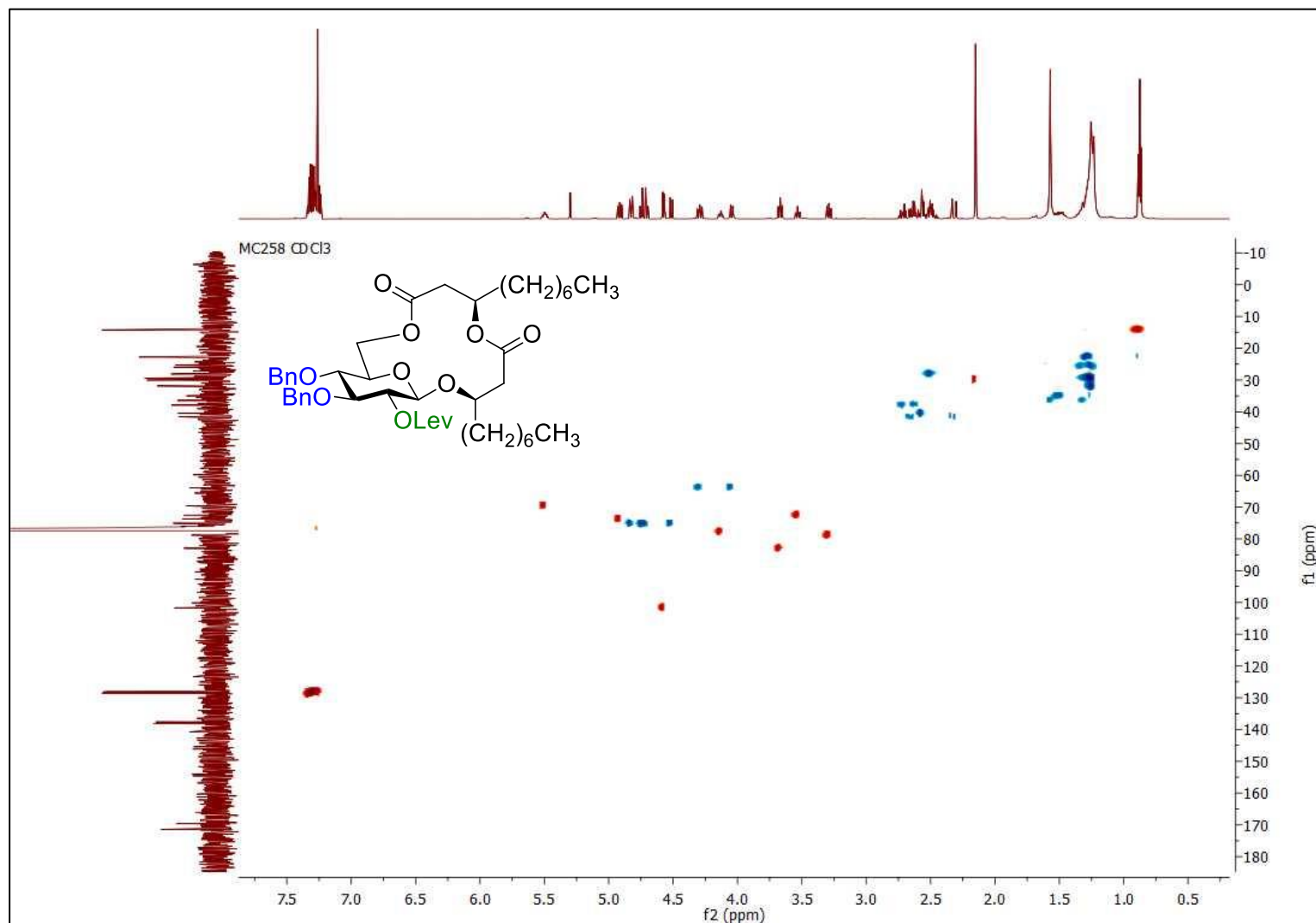
Figure S78 | HSQC NMR spectrum ( \text{CDCl}_3 , 600 MHz) of macrolide 23 .
