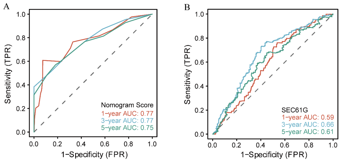
Figure S1. Time-dependent ROC analysis. Time-dependent ROCs for predicting the probability of 1-, 3-, and 5-year OS for HNSCC patients based on nomogram score (A) and SEC61G expression (B).
