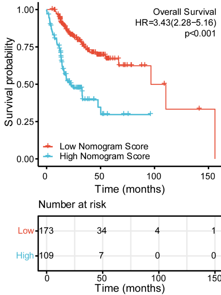
Figure S2. Kaplan–Meier curve for overall survival in HNSCC patients by nomogram score.
