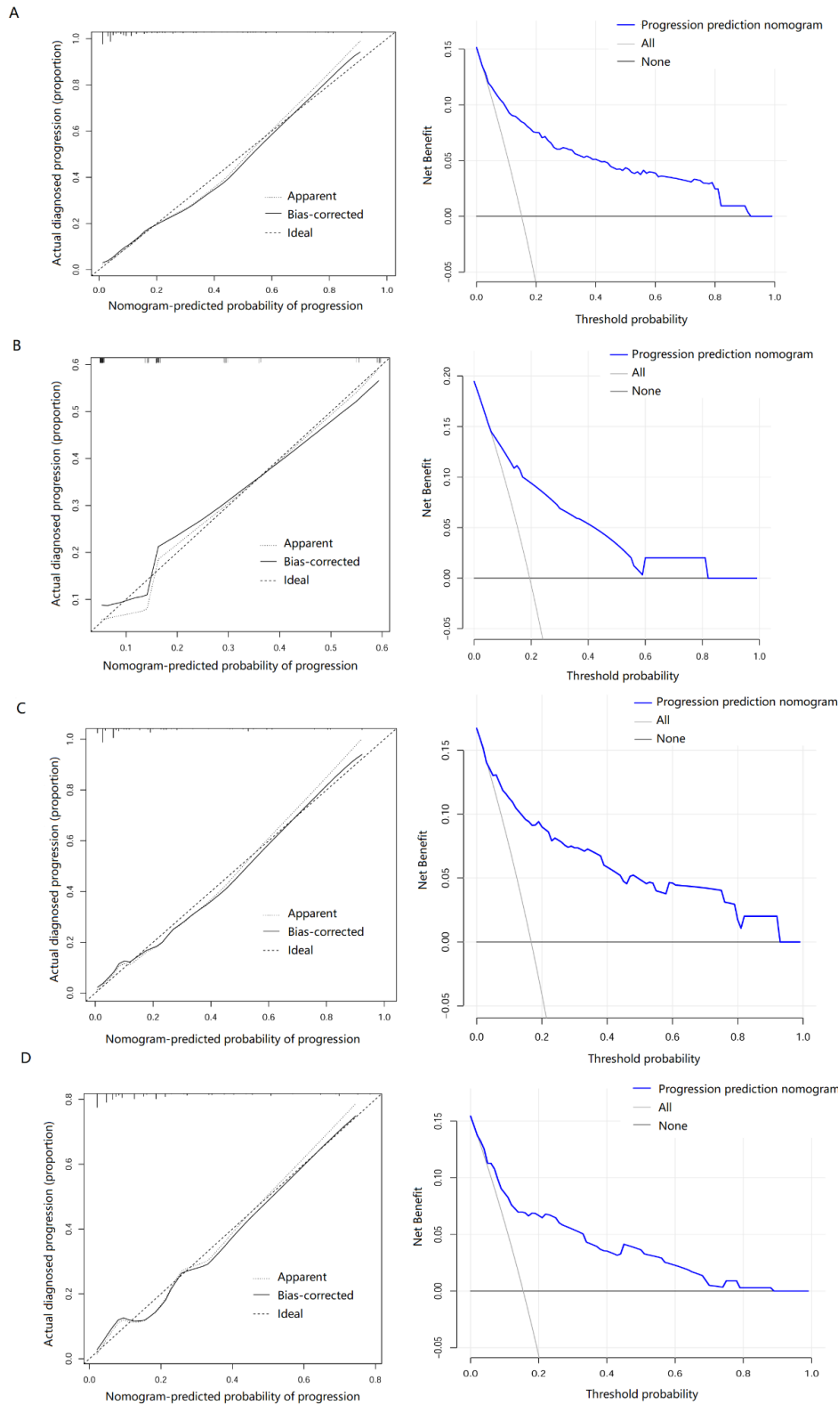
Supplementary Figure 6. Calibration curves of the nomogram prediction in patients with different molecular types metastasis risk. HR (A) positive, (B) negative, HER2 (C) positive, and (D) negative patients.
