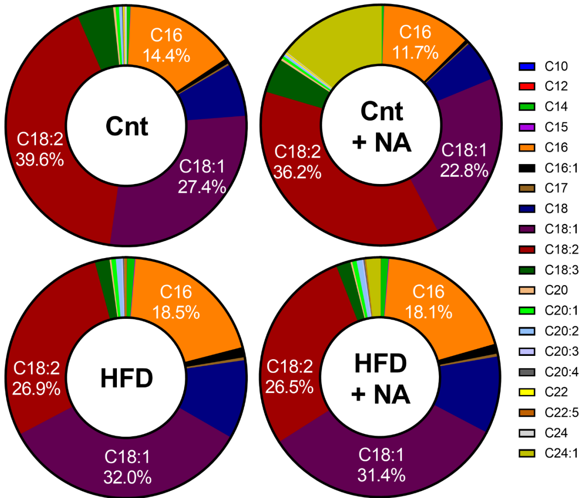
Supplemental Figure 1: Fatty acid composition of diets. The fatty acid percentages of the Cnt, Cnt+NA, HFD, and HFD+NA utilized in this study.
