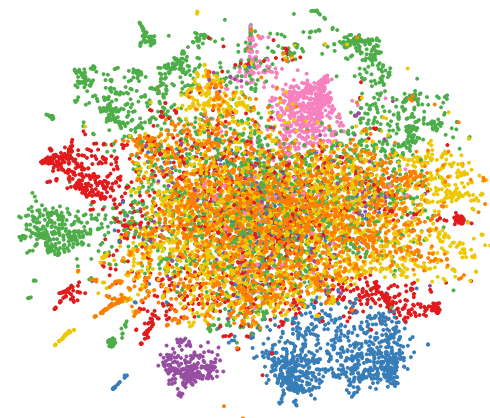
tSNE plot 06
