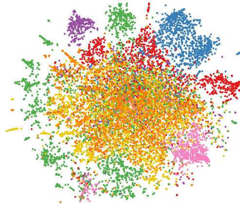
tSNE plot 17
