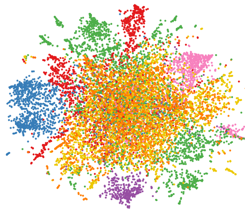
tSNE plot 20
