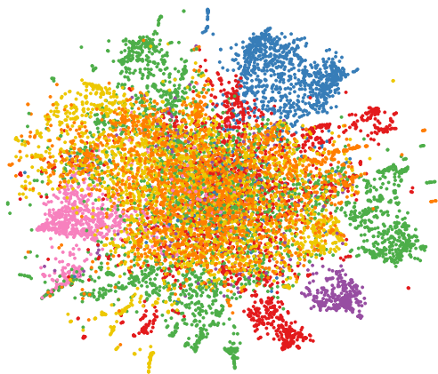
tSNE plot 07
