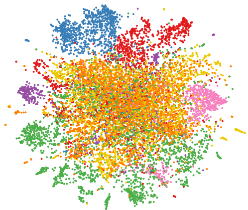
tSNE plot 25
