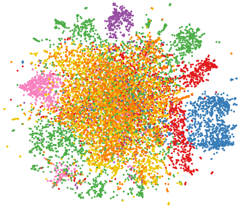
tSNE plot 16
