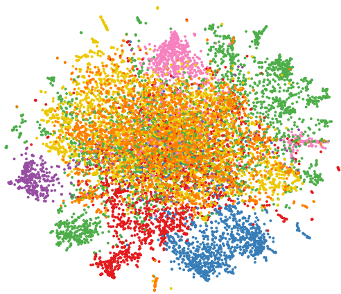
tSNE plot 01
