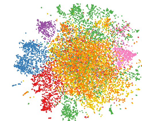
tSNE plot 24
