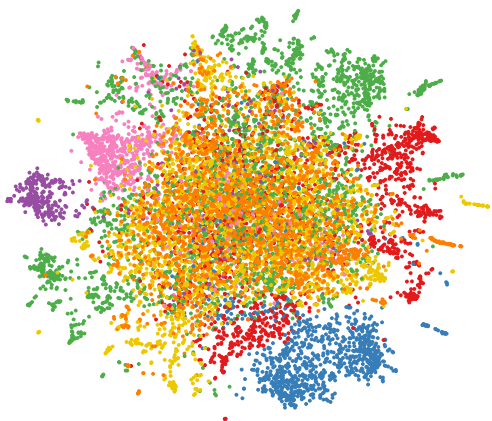
tSNE plot 10
