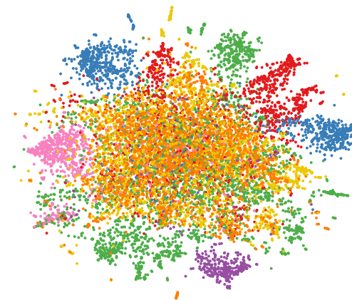
tSNE plot 21
