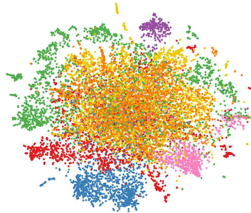
tSNE plot 14
