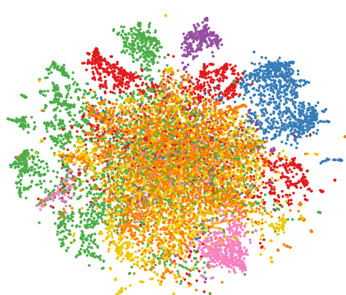
tSNE plot 11
