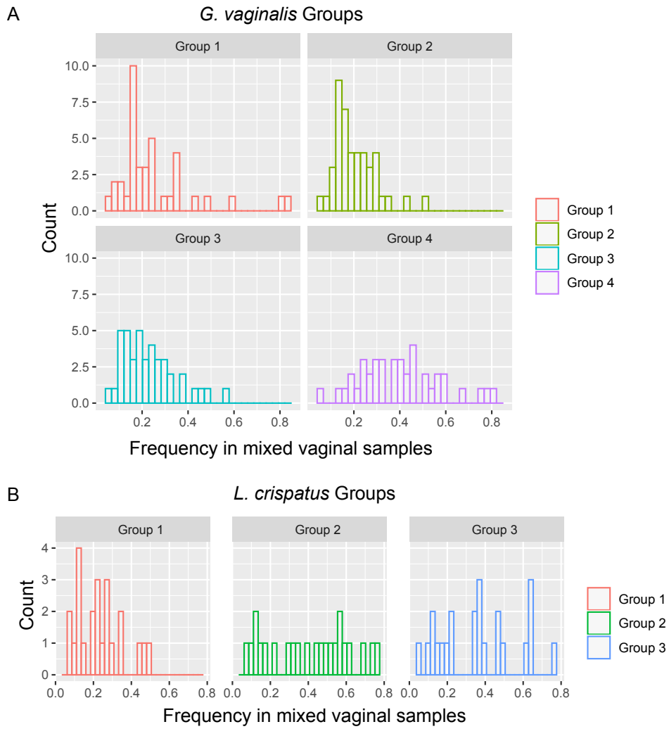
Figure S1. The relative abundance of A) G. vaginalis and B) L. crispatus groups in mixed samples based on group-specific SNPs. Each panel shows a histogram of the inferred frequency of the four G. vaginalis groups and three L. crispatus groups in vaginal samples designated as mixed populations by ADMIXTURE.
