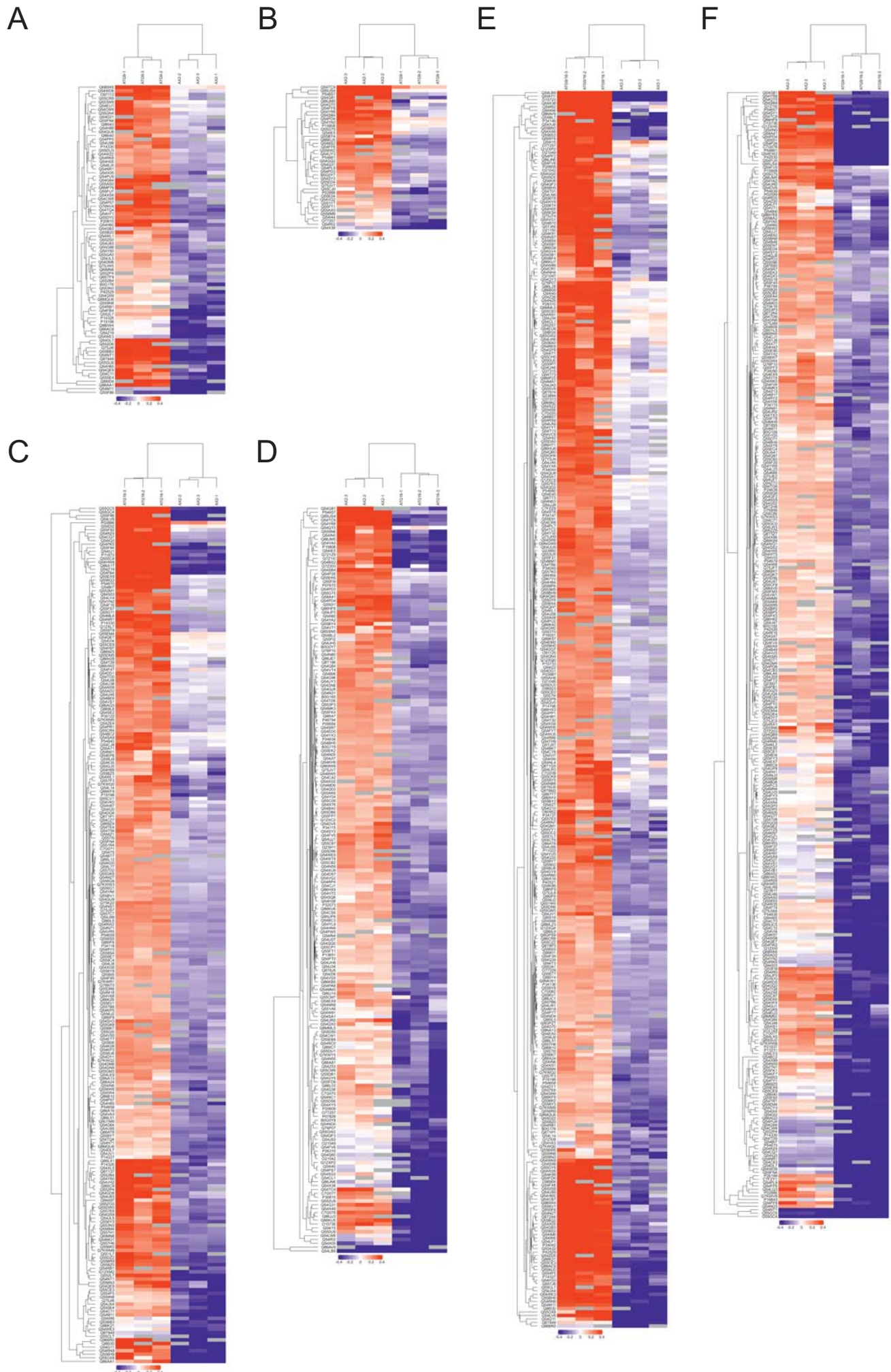
Figure S1: Hierarchical clustering analysis of DEPs of mutant strains versus AX2.
