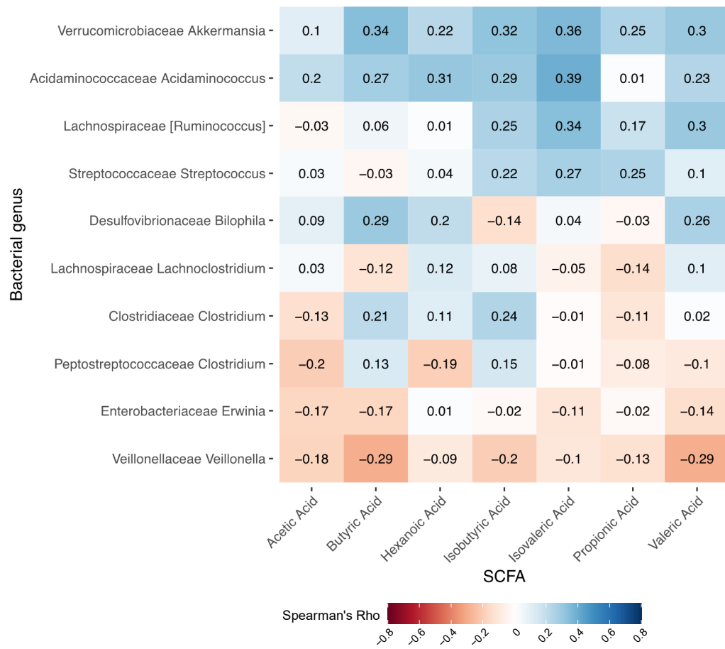
Figure S10. Spearman correlations of delivery-mode associated genera with fecal SCFA concentrations at 12 months of age.
