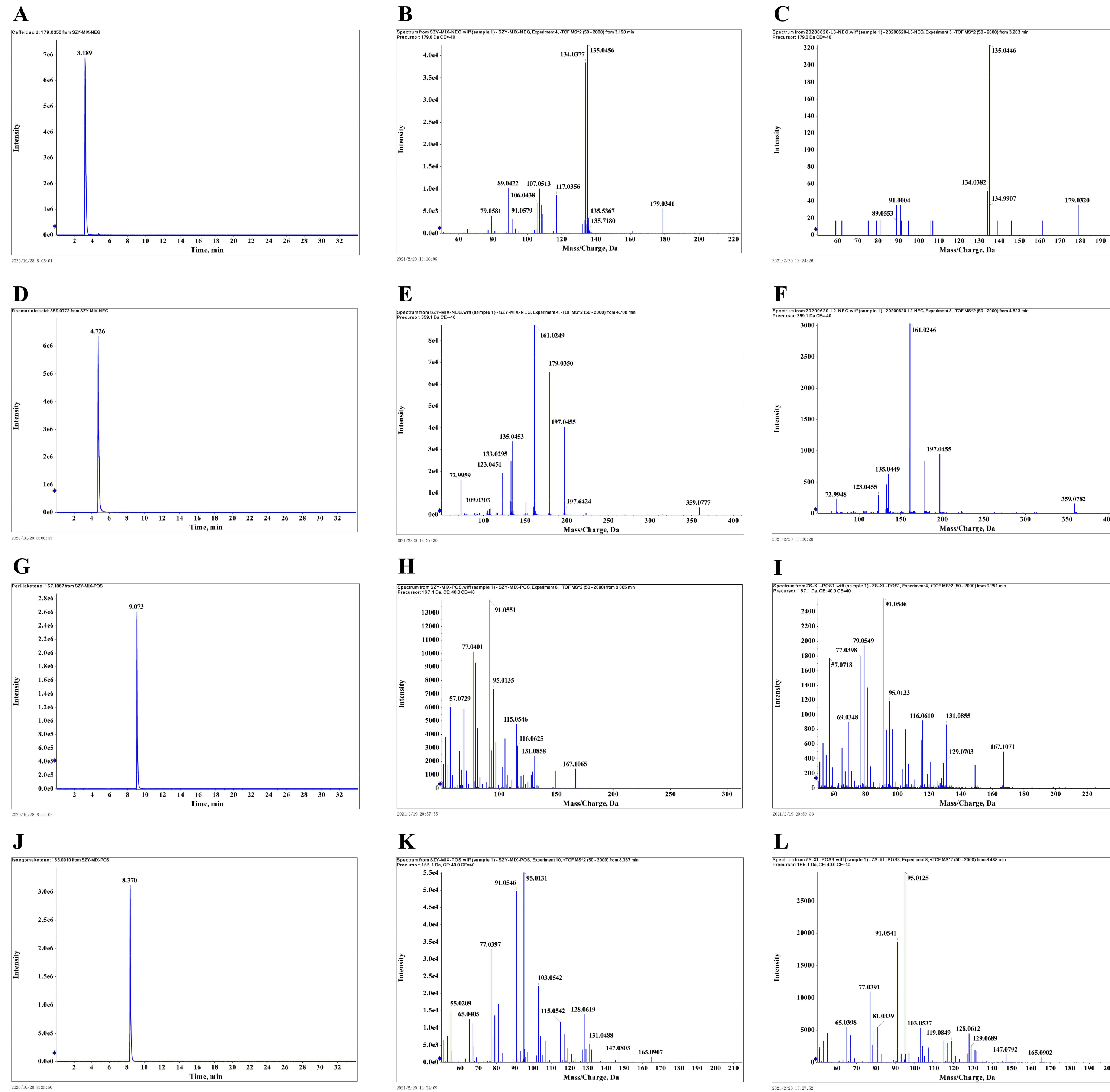
Supplementary Fig.6. LC-MS peaks of the standard mixture and mass spectra of the standard mixture and extracts; Caffeic acid standard peaks (A) and mass spectra (B), Caffeic acid extract mass spectra (C); Rosmarinic acid standard peaks (D) and mass spectra (E), Rosmarinic acid extract mass spectra (F); Perillaketone standard peaks (G) and mass spectra (H), Perillaketone extract mass spectra (I); Isoegomaketone standard peaks (J) and mass spectra (K), Isoegomaketone extract mass spectra (L).
