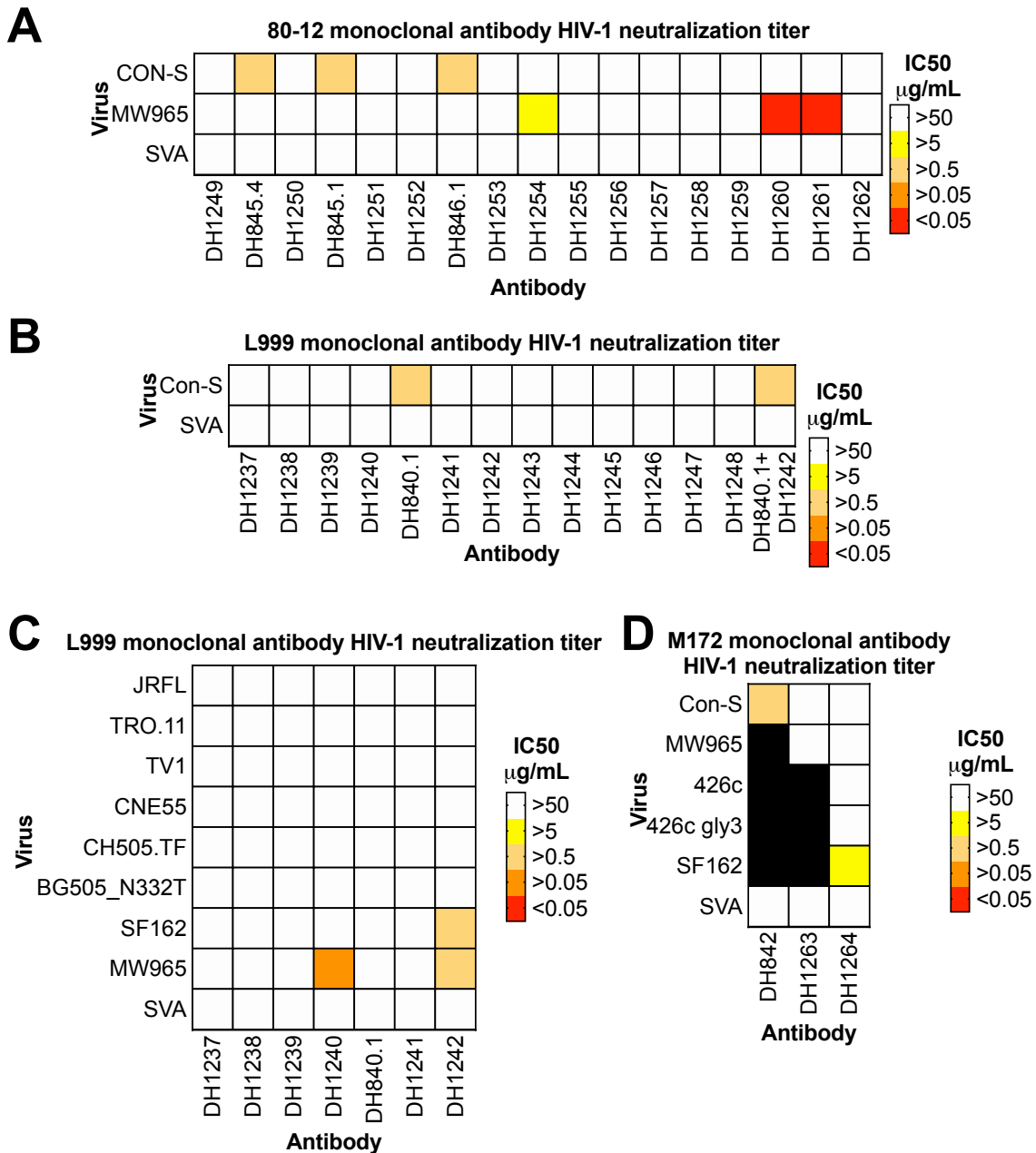
S11 Fig. HIV-1 neutralization titers for rhesus monoclonal antibodies induced by CON-S vaccination. Monoclonal antibodies were isolated from macaques (A) 80-12, (B, C) L999 and (D) M172. Each antibody was expressed and tested for neutralization activity against CON-S and other HIV-1 isolates. Neutralization titers are shown as the concentration of antibody that inhibits 50% of virus replication. Titters are color coded based on potency as indicated in the keys. Black squares show viruses not tested for a particular antibody.
