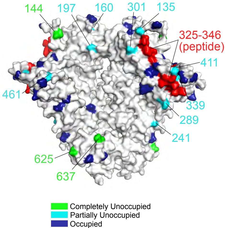
S20 Fig. Complete and partially unoccupied glycosylation sites in CON-S gp140. This figure shows the glycan sites that were found to be completely unoccupied (green) or partially unoccupied (cyan) in CON-S gp140 CFI, using data from Go et al. 53 . Other glycan sites found to be completely occupied are shown in dark blue. The site of DH840.1 contact in V3-C3 (positions 325-346) is shown in red. The crystal structure of X1193 trimer is used (PDB: 5FYJ) with hypervariable loops truncated to match those of CON-S.
