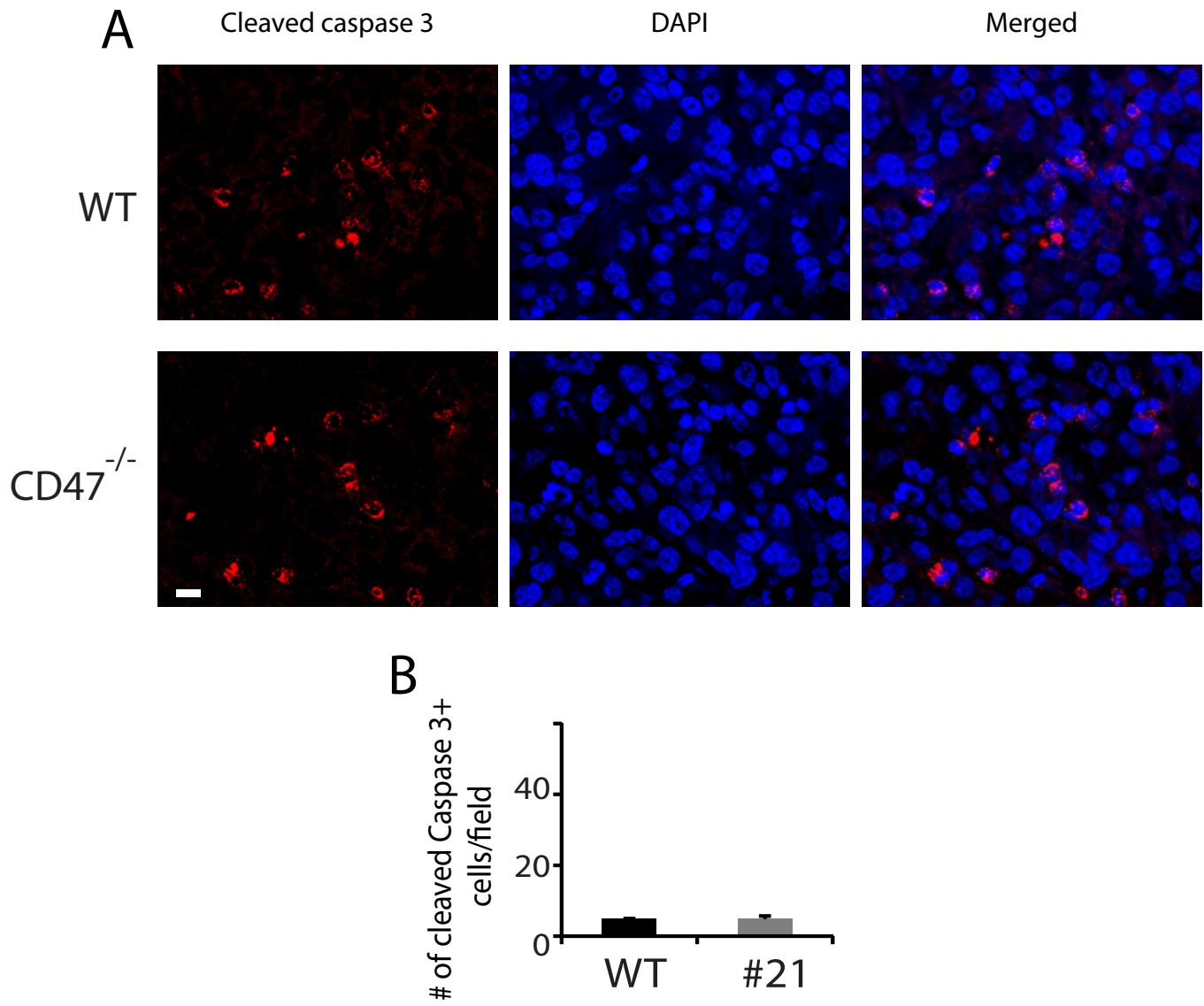
Figure S1. A. Cleaved caspase 3 staining in CD47 WT and CD47 KO xenografts. B. Quantification of the staining showed no difference between these two groups. Bar=20 \mu m. N=8.
