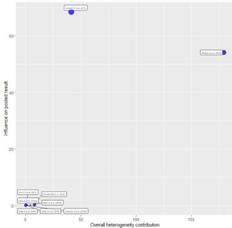
Fig. S4a. Baujat plot for studies included in the meta-analysis of pfhrp2 deletions among samples from health facilities.
