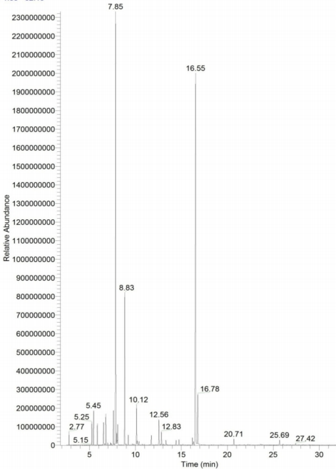
Supplementary Figure S1. Gas chromatography/mass spectroscopy spectrum of Thymus vulgaris L. essential oil native from Bosnia and Herzegovina
