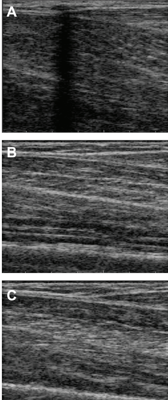
Supplemental Figure 1. Examples of image characteristics that produced poor tracking results. A) acoustic shadow, B) aponeuroses do not converge, C) more than one 'Y' shape on superficial aponeurosis
