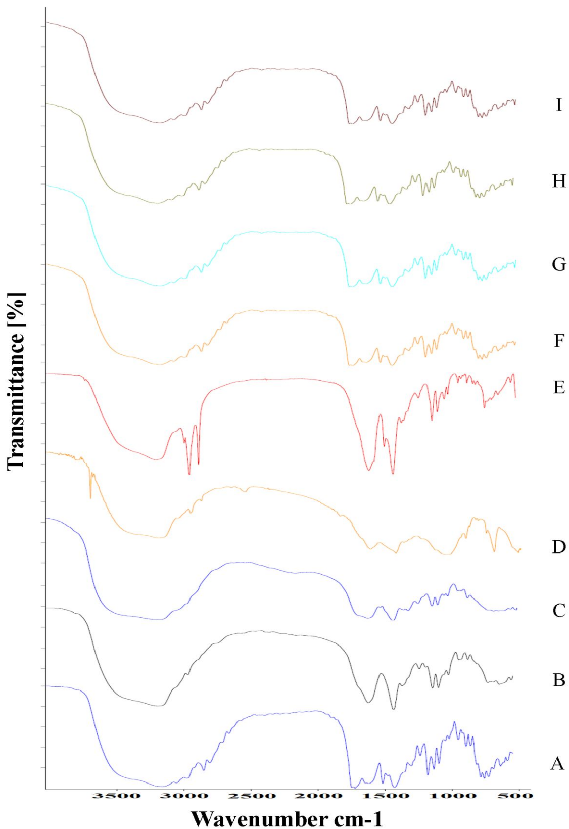
Figure S1. FTIR spectra of pure drug and tablet components. (A) Drug (Domperidone); (B) Avicel-112; (C) PVP K30; (D) Talc; (E) Magnesium stearate; (F) Drug with avicel-112; (G) Drug with PVP K30; (H) Drug with talc; (I) Drug with magnesium stearate
