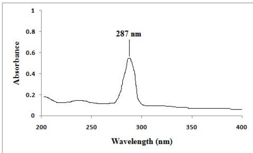
Figure S2. UV absorption maxima of domperidone
