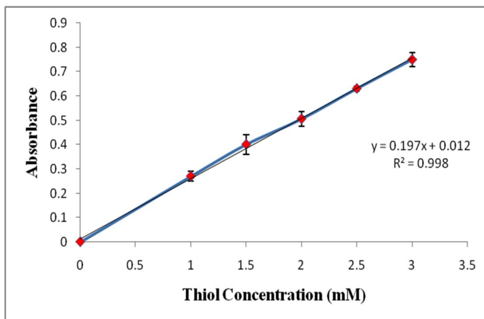
Figure S3. Standard plot of thioglycolic acid
