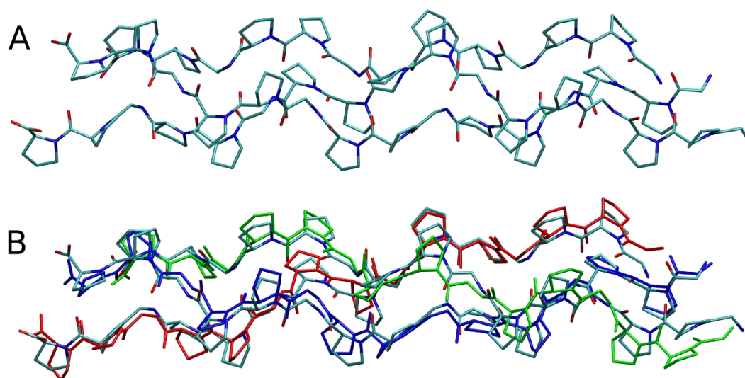
S1_Fig. (A) Structure of a folded triple helix peptide of 3 x (Gly-Pro-Pro) 5 sequence. (B) Superposition of crystal structure (light blue) and final peptide (each chain in different color) after folding simulation.
