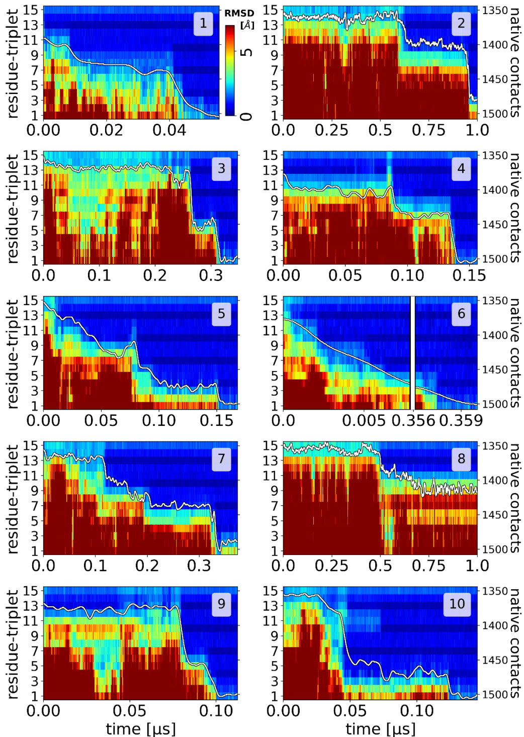
S4 Fig. RMSD of residue triplets of all WT simulations (see Fig. 1 in manuscript). Each simulation starts from an unfolded collagen peptide with an already formed nucleus at the C-terminus (top). Each labelled stripe (1-15) in the central plot represents a residue triplet (one residue with the same number of each strand, e.g. 3 Pro with the same number that are spatially close in the native state) along the three strands. The RMSD of each residue triplet relative to the native folded structure is indicated by a color-code (color bar in the first plot). A blue color represents sampled states close to native, whereas red color corresponds to an unfolded triplet structure. The y-axis on the right side of the plot represents the number of native contacts between the three strands (white line in the plot). All simulation ran for 1 \mu s. To present the folding process in detail the time range of each graph was adjusted.
