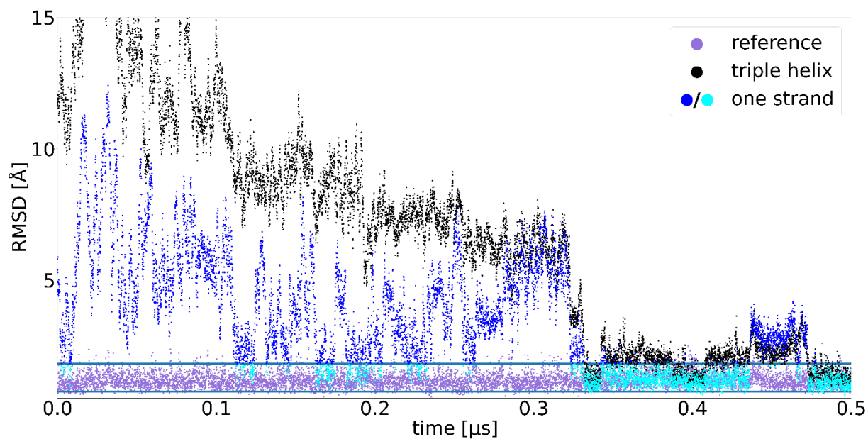
S6_Fig. Root mean square deviation (RMSD) of individual chains during triple helix folding. For an example folding simulation the RMSD (non-hydrogen atoms) with respect to the native triple helical conformation vs. time is indicated (black curve: RMSD vs time of complete structure; violet: simulation starting from the triple helix; dark/light blue: RMSD of separate chains).
