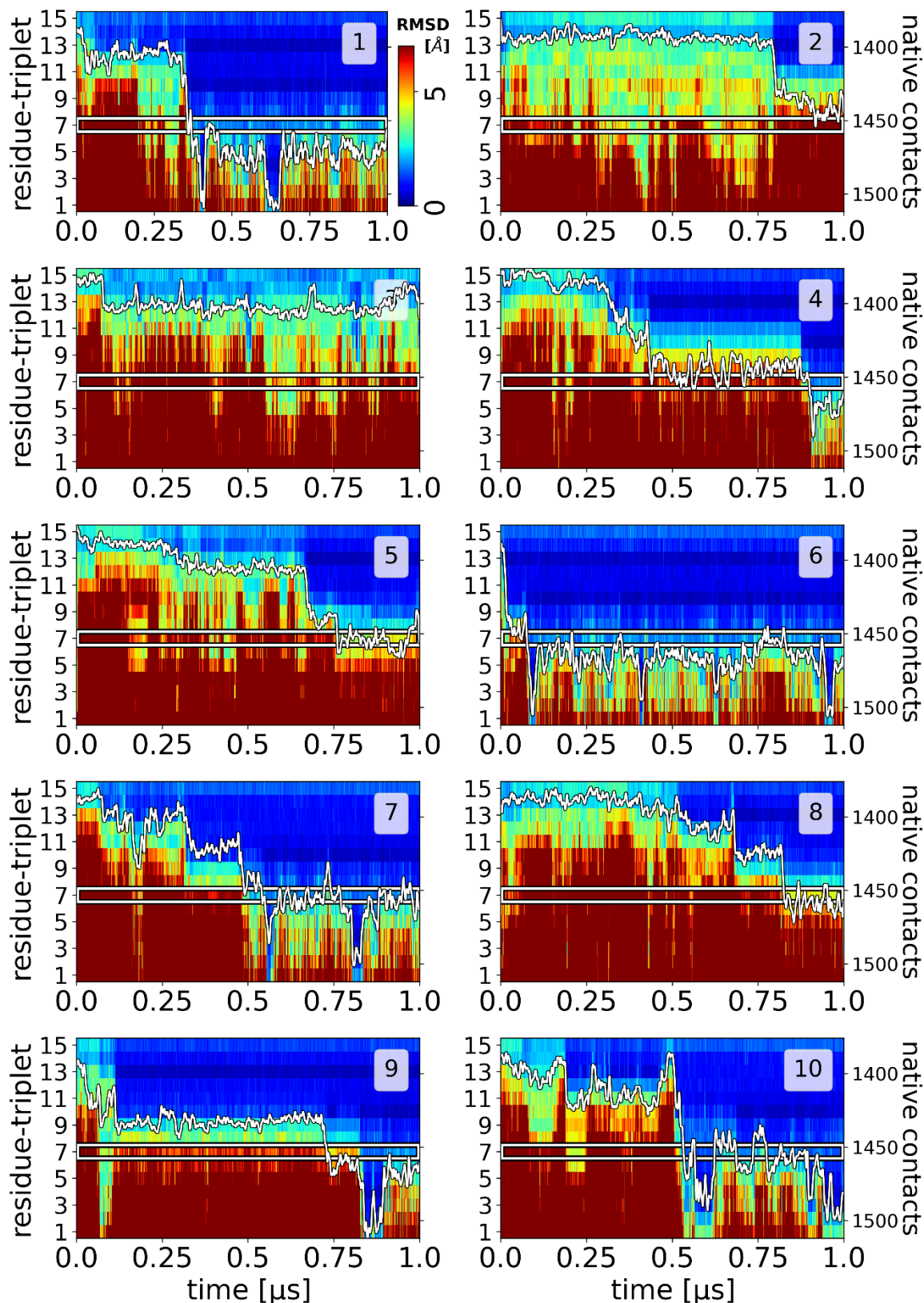
S11_Fig. RMSD of residue triplets of all simulations with three mutations G7abcA (indicating position 7 in each chain A,B,C; marked by white frame). The simulation starts from an unfolded collagen peptide with an already formed nucleus at the C-terminus (top). Same as legend of S9_Fig.
