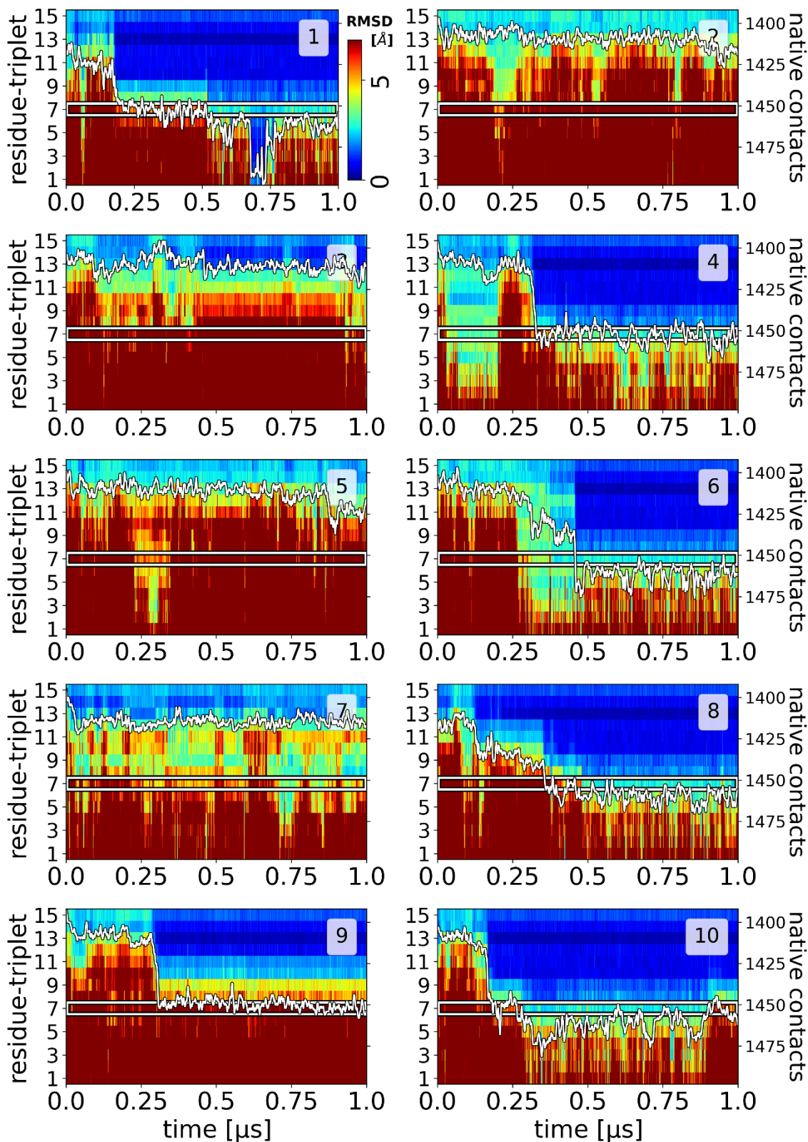
S12_Fig. Same as S11_Fig but for simulations with three mutations G7abcT (marked by white frame).
