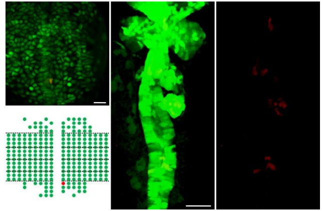
R-P-c1r1 (n=5)
