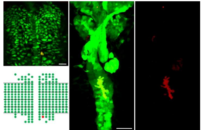
R-P-c2r2 (n=5)
