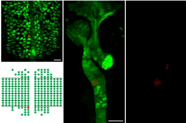
L-P-c1r1 (n=7)
