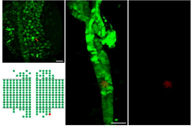
R-P-c5r3 (n=5)
