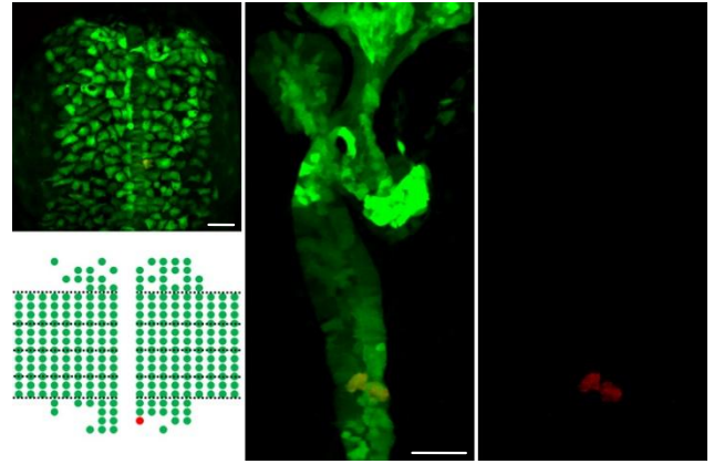
R-P-c1r3 (n=5)
