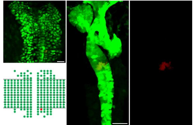
R-P-c2r1 (n=5)
