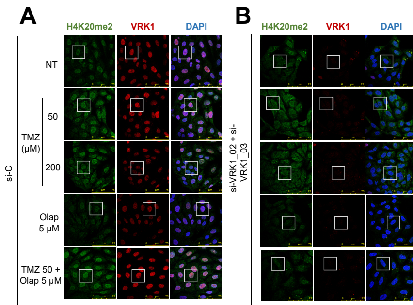
Figure S7. Effect of VRK1 knockdown on H4K20me2 induced by TMZ and olaparib in LN-18. A. Effect of siControl on H4K20me2c induced by TMZ, olaparib and the combination of both drugs shown by IF. B. Effect of siVRK1-02 and siVRK1-03 on H4K20me2 induced by TMZ, olaparib and their combination shown by IF. NT: no treatment. Field images from Figure 4. Squares indicate the cells shown in Figure 4.
