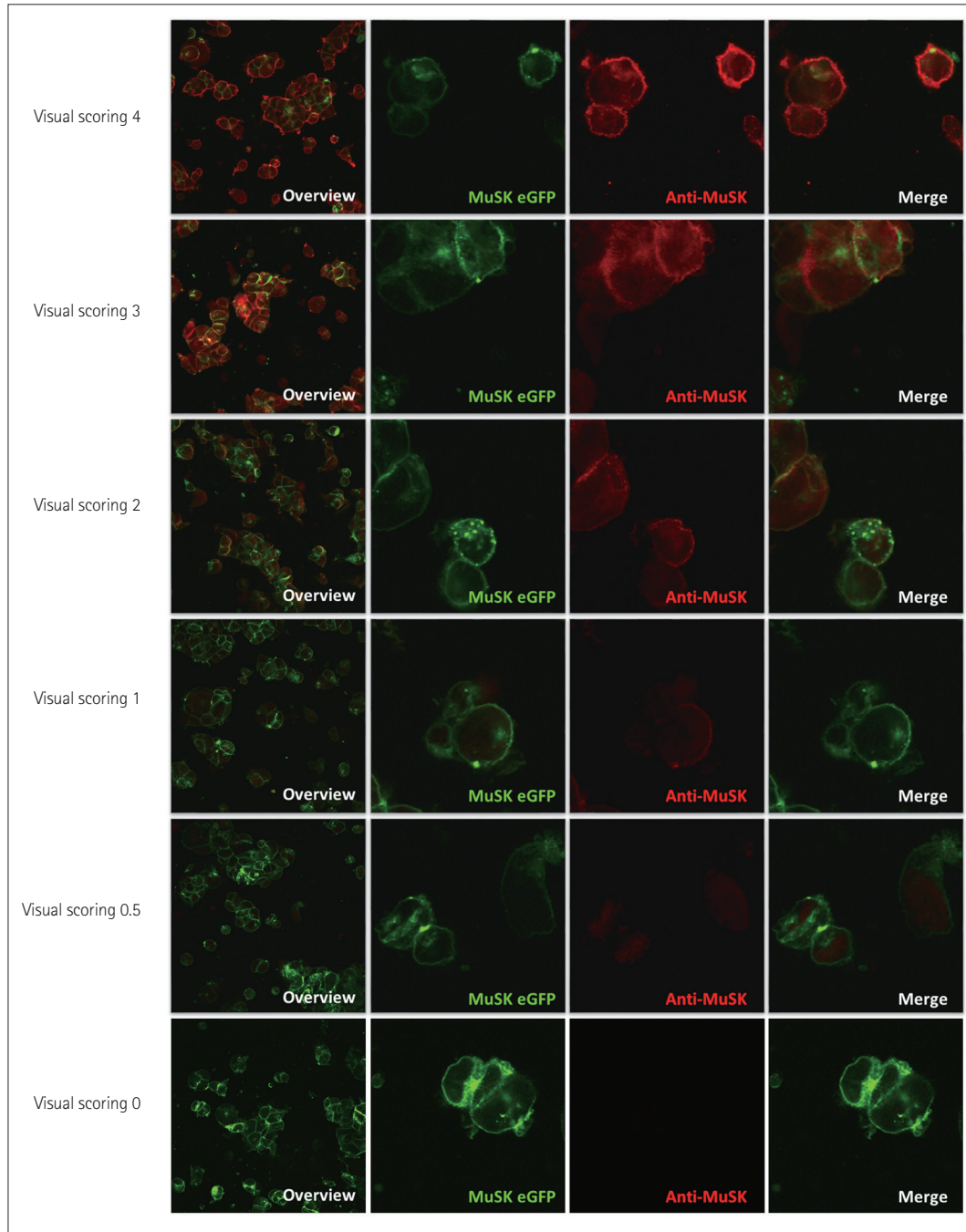
Supplementary Fig. 1. The representative images of the CBA in each level of visual scores. Anti-human IgG antibody binding (red fluorescence) is observed along the cell surface which co-localizes with MuSK-GFP expressed on the surface of HEK293 cells (green fluorescence). CBA: cell-based assay, HEK293: human embryonic kidney 293, MuSK-GFP: muscle-specific tyrosine kinase fused to green fluorescent protein
