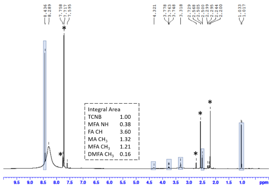
Figure S18. Full ^1\text{H} NMR spectrum of TC precursor in d_7 -DMF/ d_6 -DMSO (4:1) after 28 days aging. Asterisks denote peaks of interest: Peaks at 7.72 ppm and 2.20 ppm are assigned to the CH of FA and CH 3 of MA respectively. Emerging peaks at 2.57 ppm and 7.76 ppm are assigned to CH 3 and NH of MFA respectively, with the peak at 2.73 assigned to the CH 3 of DMFA. Integral values, referenced to the TCNB standard as 1.00, are shown in the inset box.
