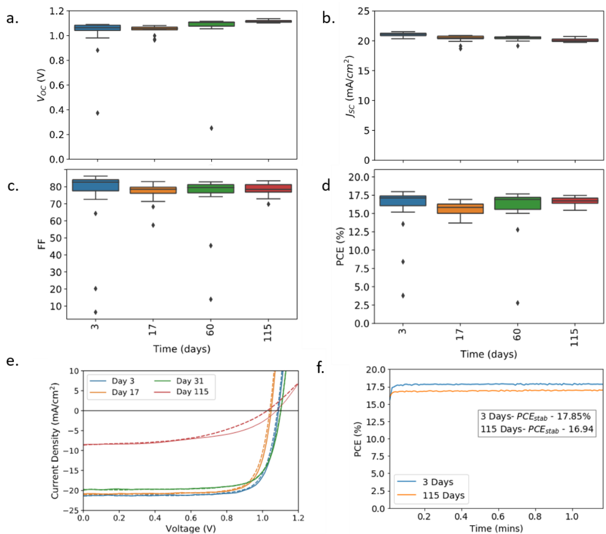
Figure S6. LT-aged TC-DMSO device metrics. (a) V_{oc} , (b) J_{sc} , (c) FF, (d) PCE, (e) J-V curves and (f) stabilised power output measurements for the best performing devices.
