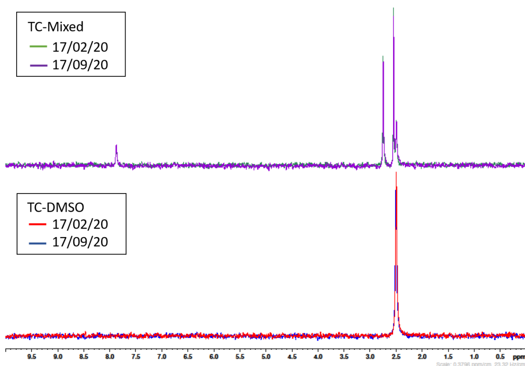
Figure S14. ^2\text{H} spectra of TC solutions dissolved in d_7\text{-DMF}/d_6\text{-DMSO} (4:1) (above) and d_6\text{-DMSO} (below) before and after 6 months storage at RT under nitrogen. Peaks at 2.5 ppm are assigned to d_6\text{-DMSO} and those at 2.55 ppm, 2.75 ppm and 7.87 ppm are assigned to d_7\text{-DMF} .
