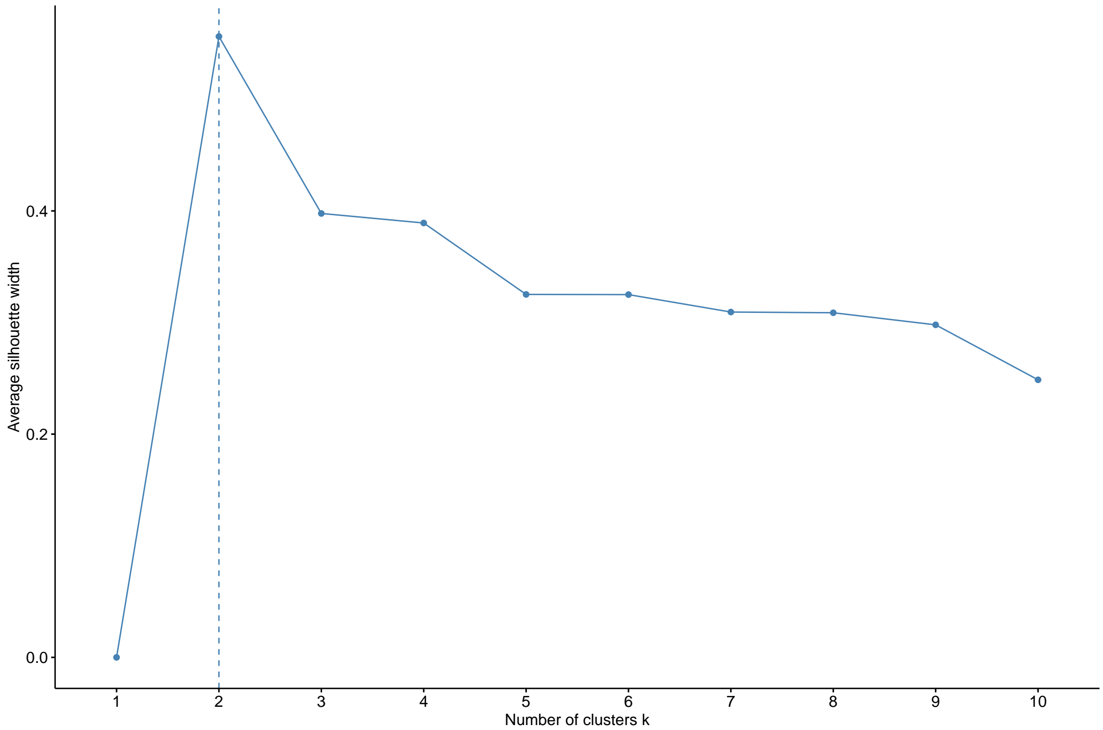
Optimal number of clusters Bones – Total
