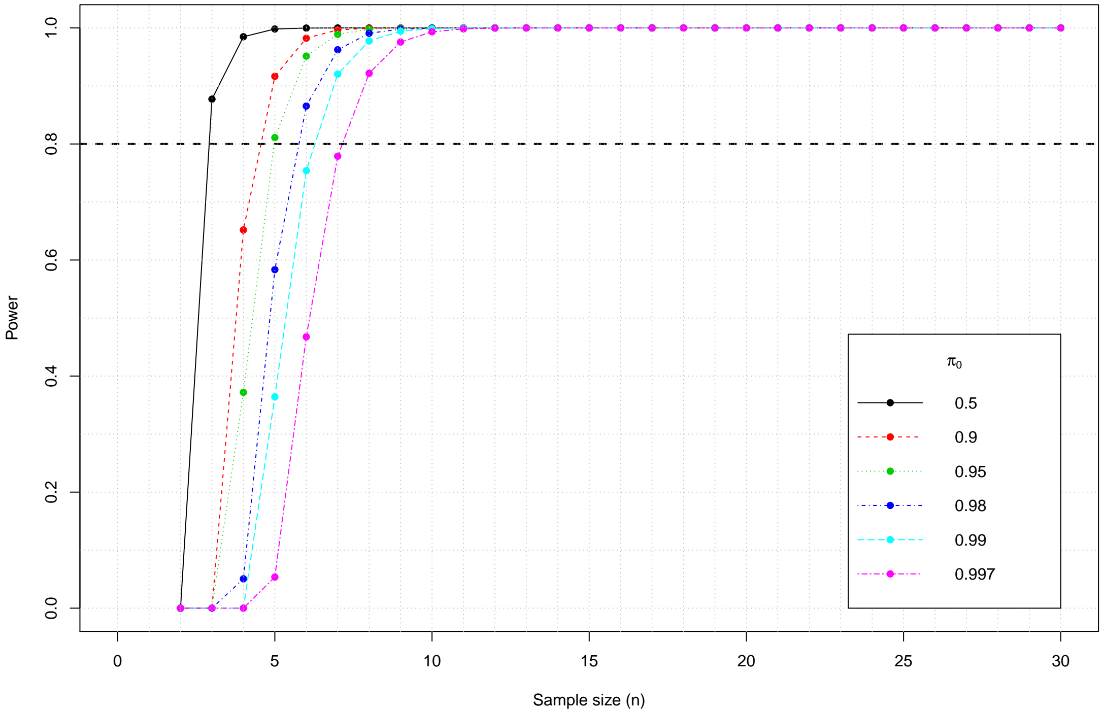
Power vs. sample size with \text{fdr}=0.05 and \Delta/\sigma = 3.5251
