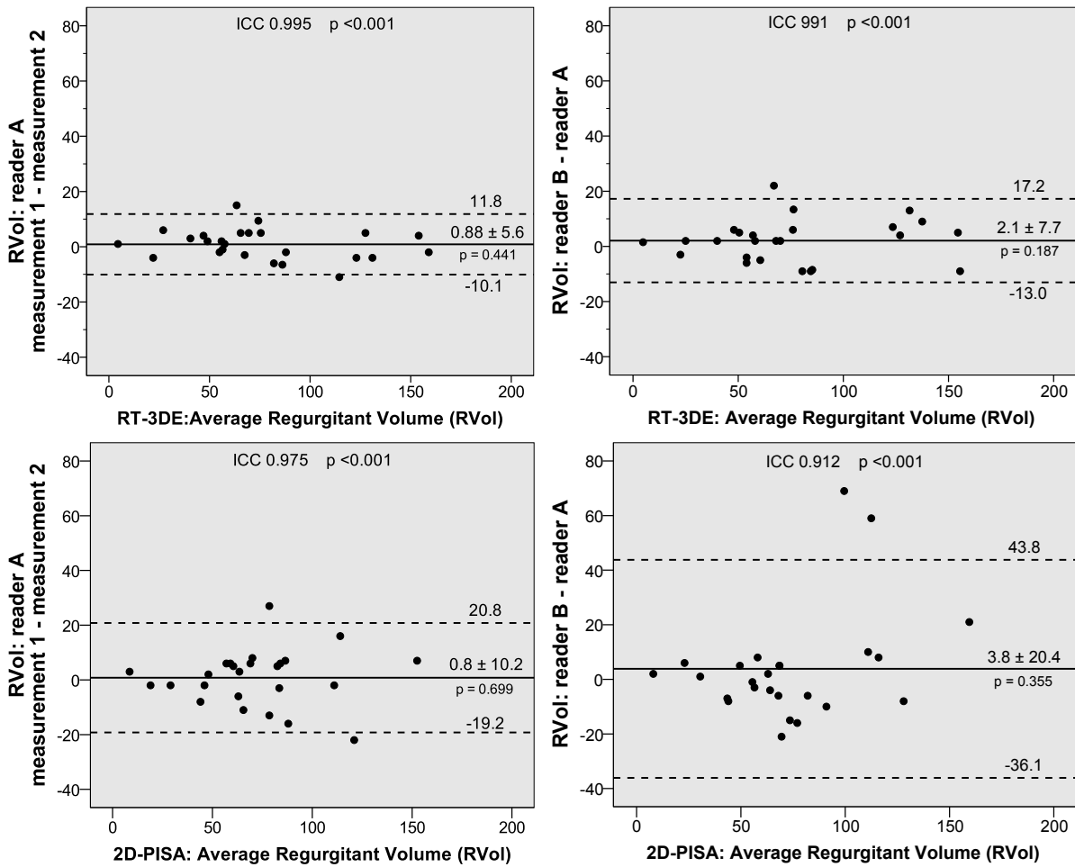
Online Resource 4- Bland-Altman plots for regurgitant volume (RVol) measurement: intra- (left panels) and inter-observer (right panels) variability with 3D-PISA (top panels) and 2D-PISA method (bottom panels). ICC = intraclass correlation coefficient.
