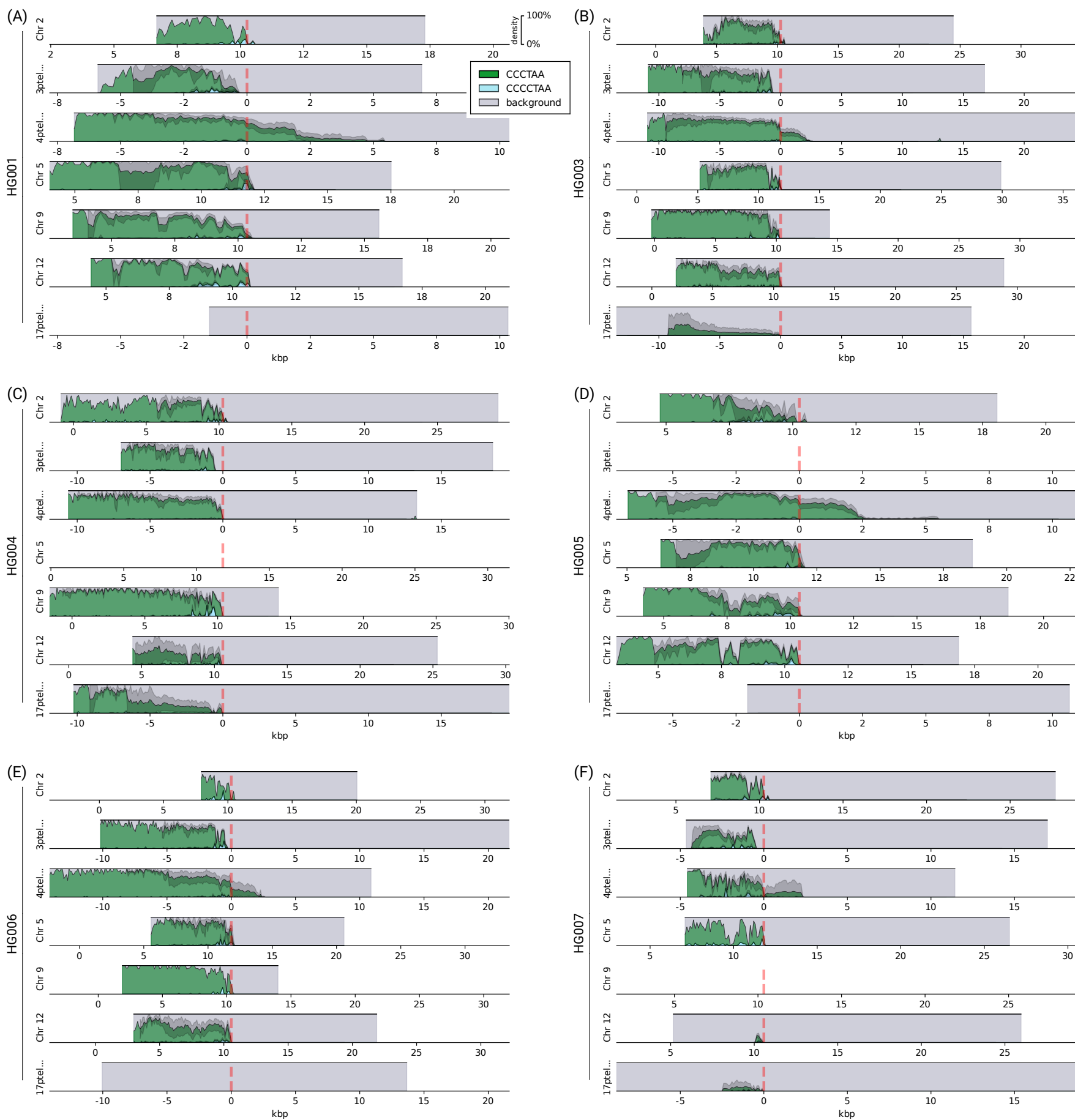
Supplemental Figure S2. Densities of the top two enriched motifs at ends of chromosomal p arms of datasets (A) HG001, (B) HG003, (C) HG004, (D) HG005, (E) HG006, and (F) HG007. Only the arms covered by at least 25 reads across all datasets are displayed. Genomic coordinates are given in kbp. Vertical red dashed lines denote the position of the boundary of the annotated telomeric tract.
