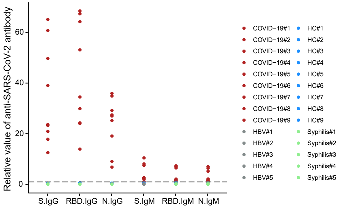
Supplementary Figure S1. Validation of the performance of commercial kits. The x-axis represents the antibody category, and the y-axis represents relative value of anti-SARS-CoV-2 antibody.
