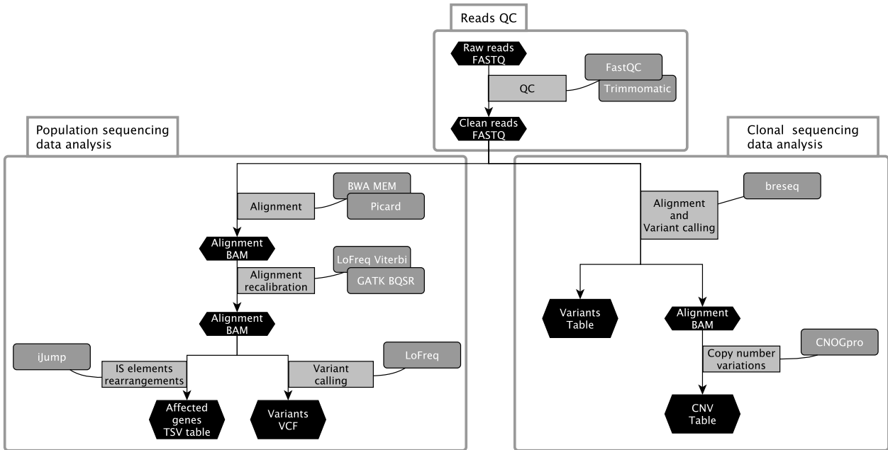
Supplementary Figure 3. Computational pipeline for a primary analysis of population sequencing data. Data shown in black hexagons. Processes and software shown in rectangles and rounded rectangles respectively. Frames indicate aims of the parts of the analysis.
