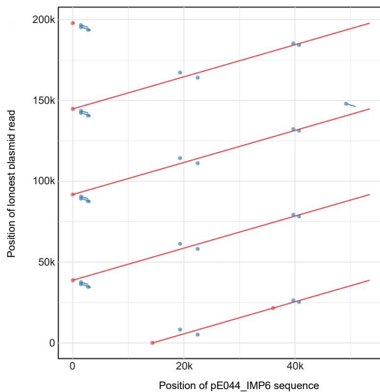
FIG S2. Plasmid multimerization observed by MinION. The longest read (198 kb) obtained from ultra-long sequencing of isolate E044 was mapped 3.7 times serially to pE044_IMP6 (53 kb) in the forward strand. The colors of the lines show strand direction of the longest read (198 kb) compared with pE044_IMP6, as forward (red) and reverse (blue).
