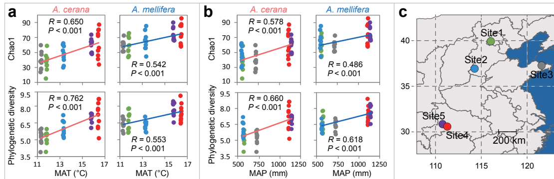
Fig. S2 Chao1 richness and phylogenetic diversity of A. cerana and A. mellifera gut bacterial communities positively correlated with mean annual temperature (MAT) and mean annual precipitation (MAP). a , Positive correlations between diversity indices and MAT. b , Positive correlations between diversity indices and MAP. c , The sampling sites.
